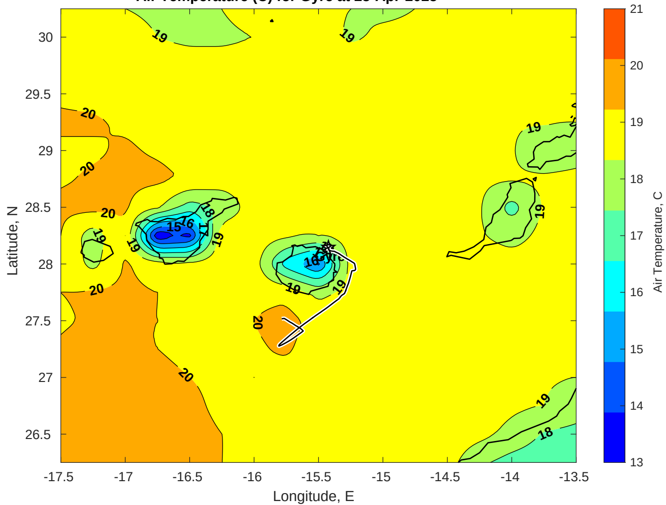
Air Temperature (C) for Gyre at 25-Apr-2025
