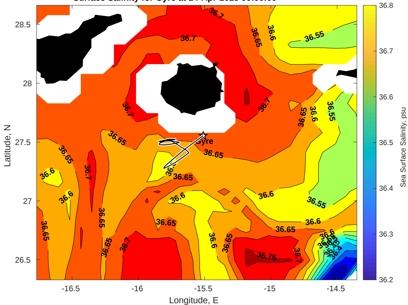
Surface Salinity for Gyre at 24-Apr-2025 00:00:00
