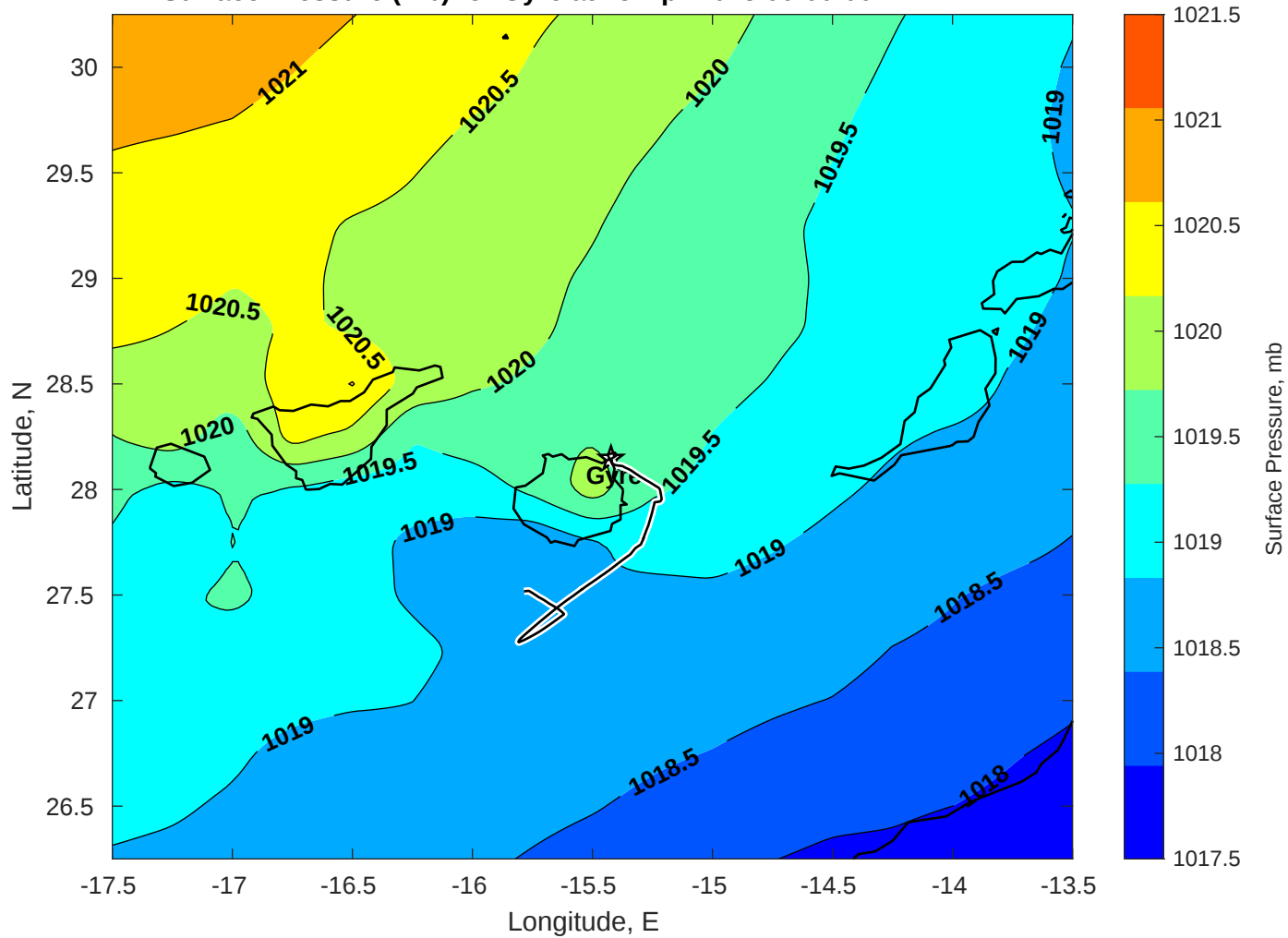
Surface Pressure (mb) for Gyre at 25-Apr-2025 00:00:00
