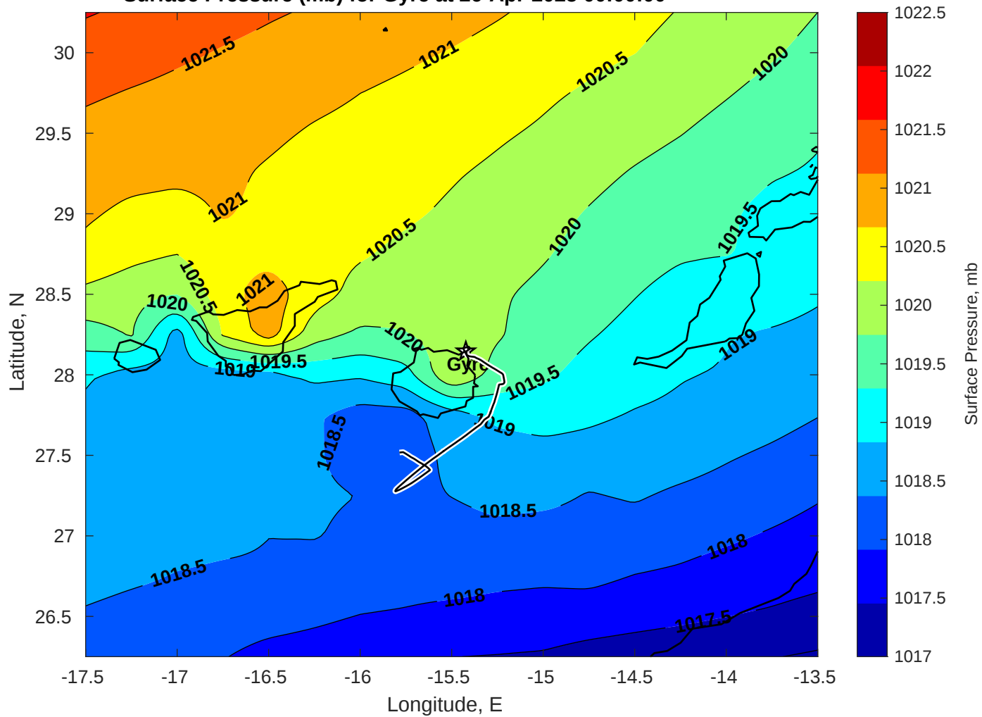
Surface Pressure (mb) for Gyre at 26-Apr-2025 00:00:00
