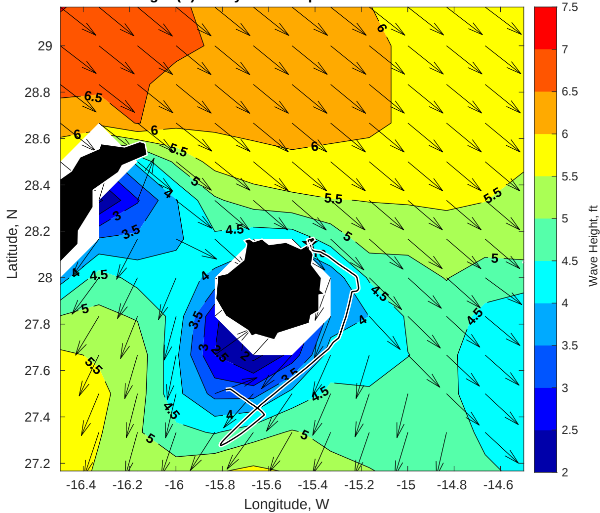
Wave Height (ft) for Gyre at 25-Apr-2025 09:00:00
