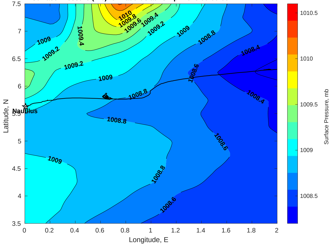
Surface Pressure (mb) for Nautilus at 25-Apr-2025 00:00:00
