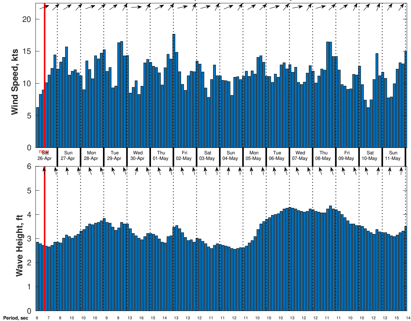
Wind & Wave Forecast for Nautilus from 25-Apr-2025 02:00:00 to 11-May-2025 02:00:00
