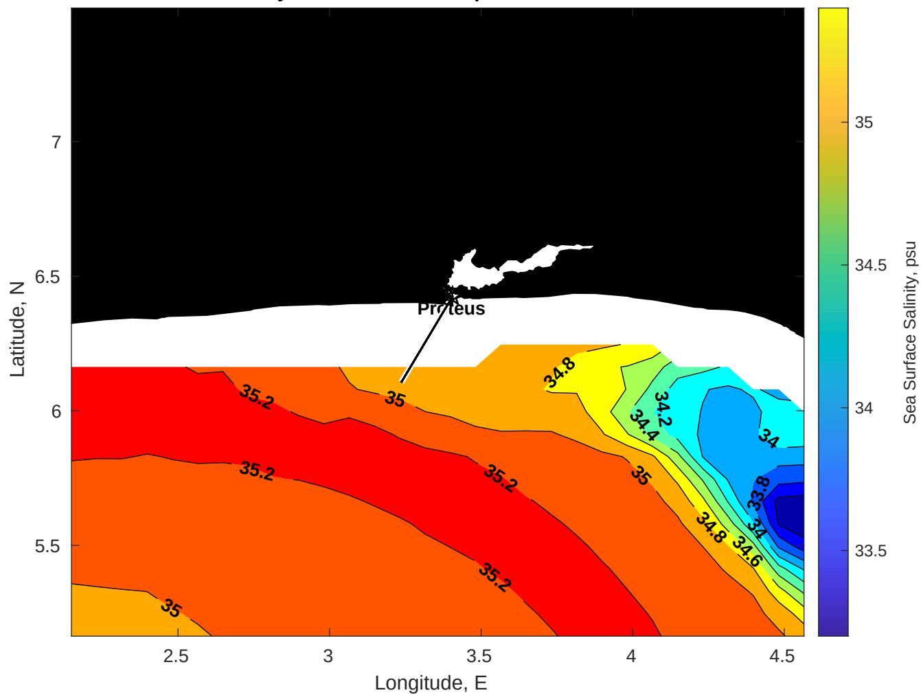
Surface Salinity for Proteus at 24-Apr-2025 00:00:00
