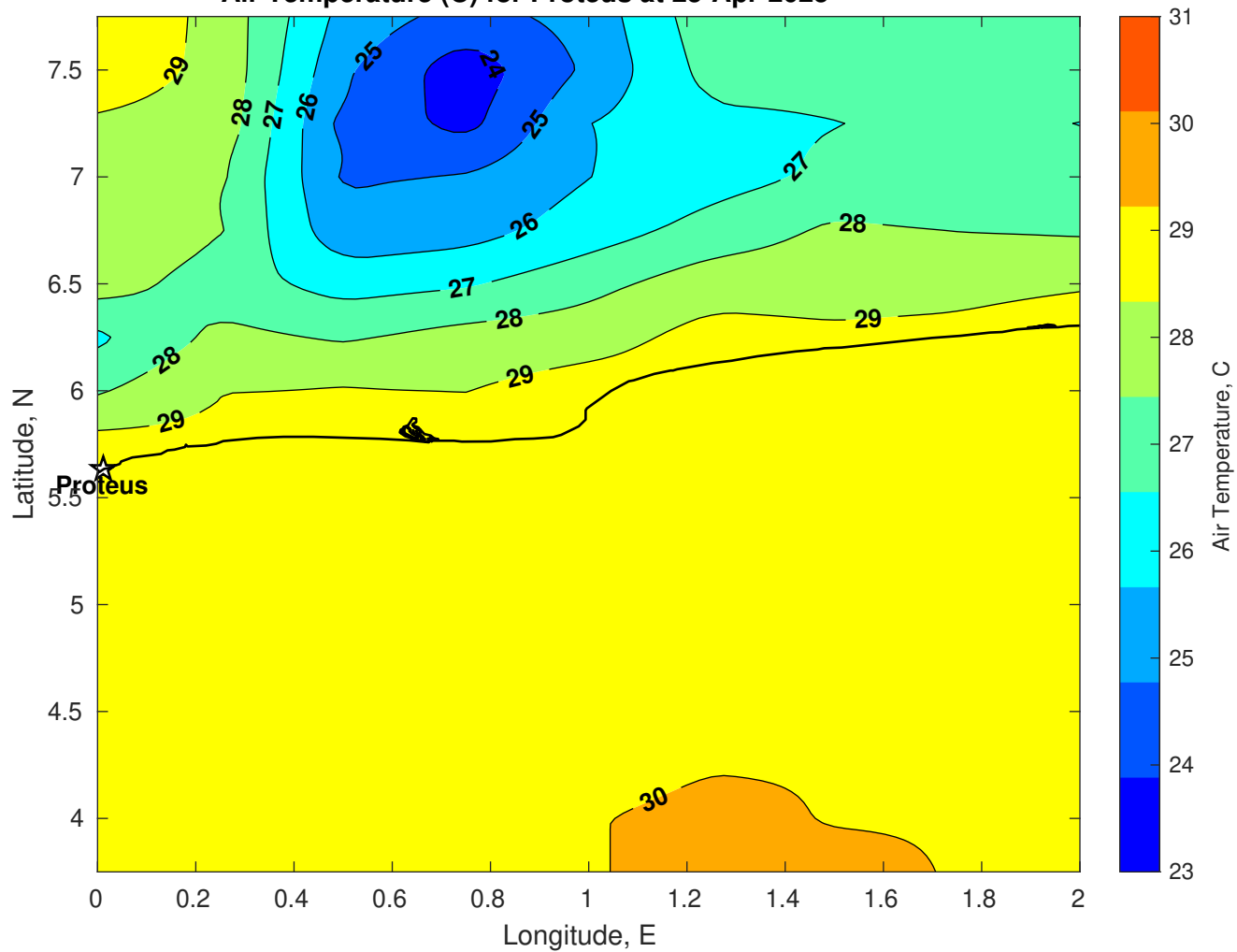
Air Temperature (C) for Proteus at 25-Apr-2025
