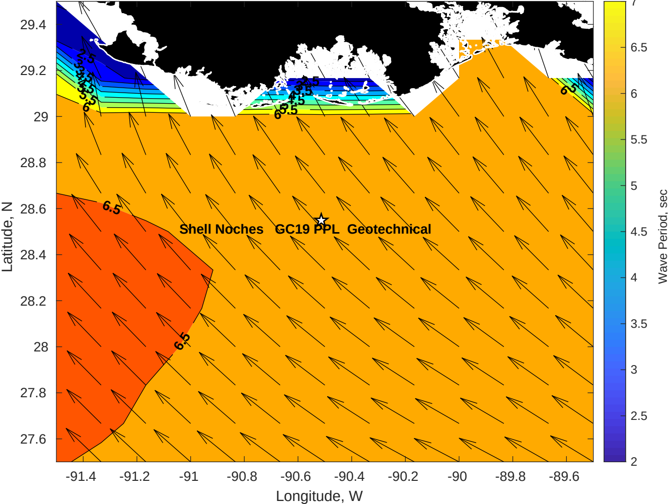
Wave Period (sec) for Shell Noches GC19 PPL Geotechnical at 25-Apr-2025 09:00:00
