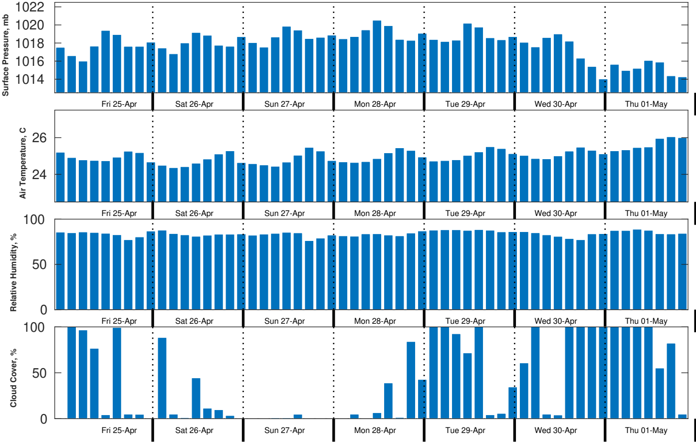
Met Forecast for Shell Noches GC19 PPL Geotechnical from 25-Apr-2025 00:00:00 to 02-May-2025 00:00:00
