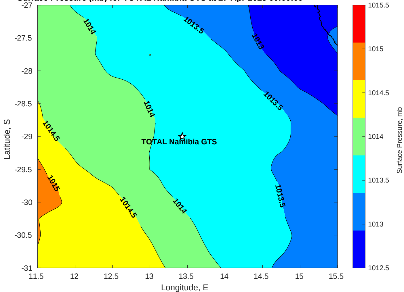
Surface Pressure (mb) for TOTAL Namibia GTS at 27-Apr-2025 00:00:00
