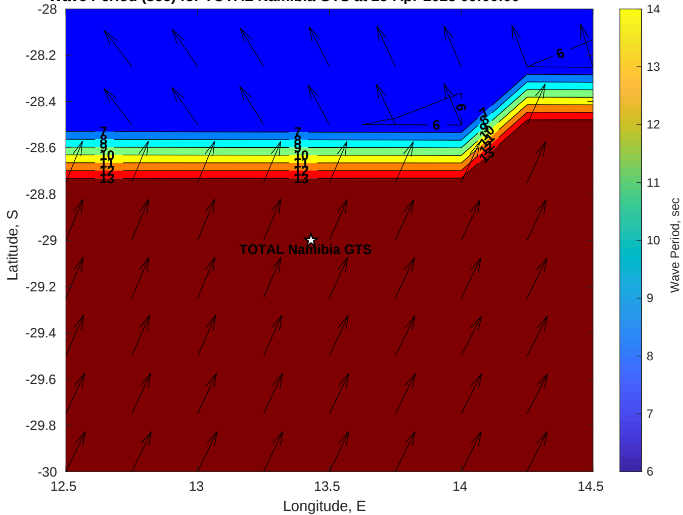
Wave Period (sec) for TOTAL Namibia GTS at 25-Apr-2025 09:00:00
