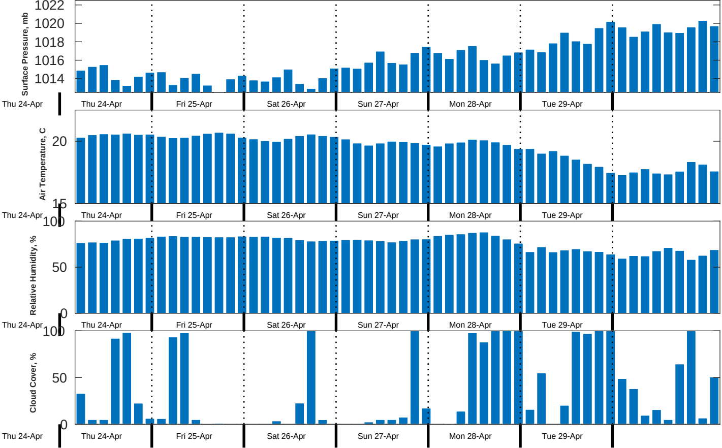
Met Forecast for TOTAL Namibia GTS from 25-Apr-2025 00:00:00 to 02-May-2025 00:00:00
