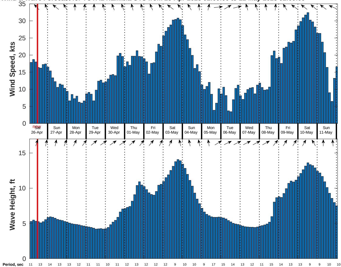
Wind & Wave Forecast for TOTAL Namibia GTS from 25-Apr-2025 02:00:00 to 11-May-2025 02:00:00
