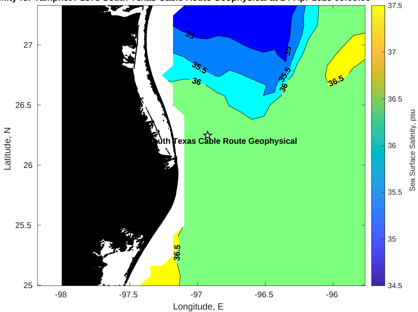
Surface Salinity for Tampnet P2378 South Texas Cable Route Geophysical at 24-Apr-2025 00:00:00
