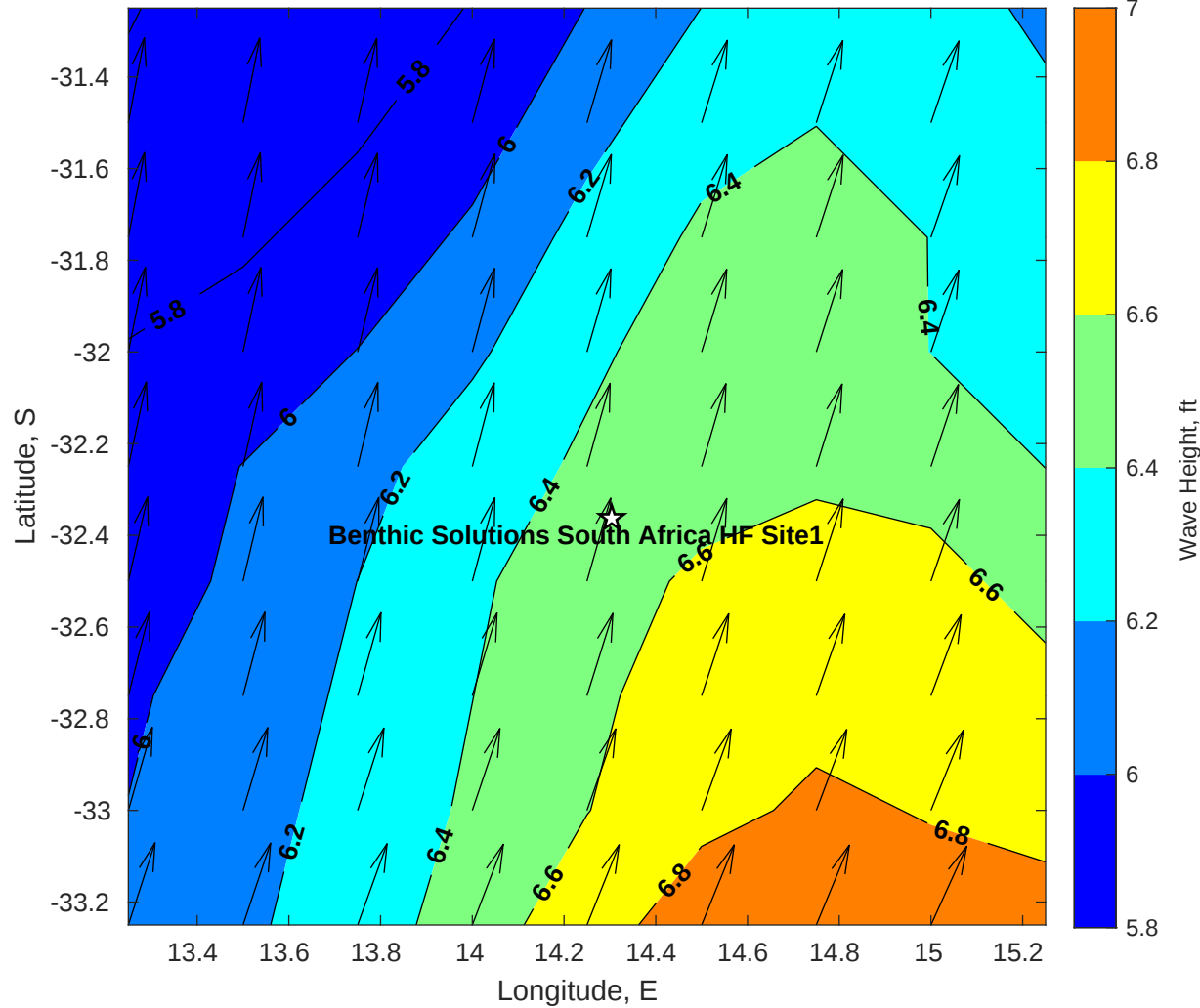
Wave Height (ft) for Benthic Solutions South Africa HF Site1 at 26-Apr-2025 09:00:00
