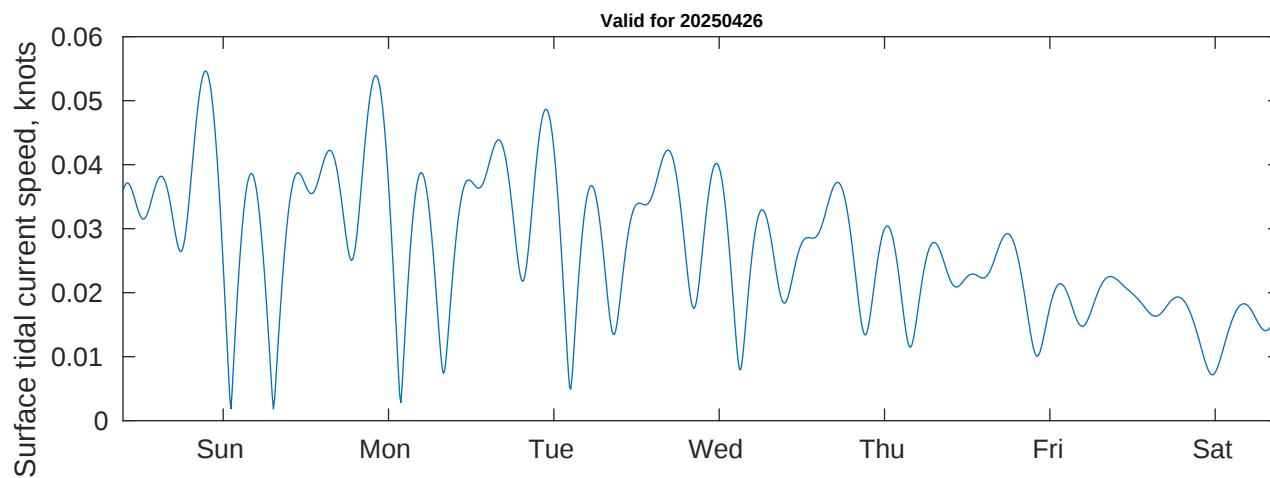
Tidal Currents and Heights for Benthic Solutions South Africa HF Site1 at 20250426
