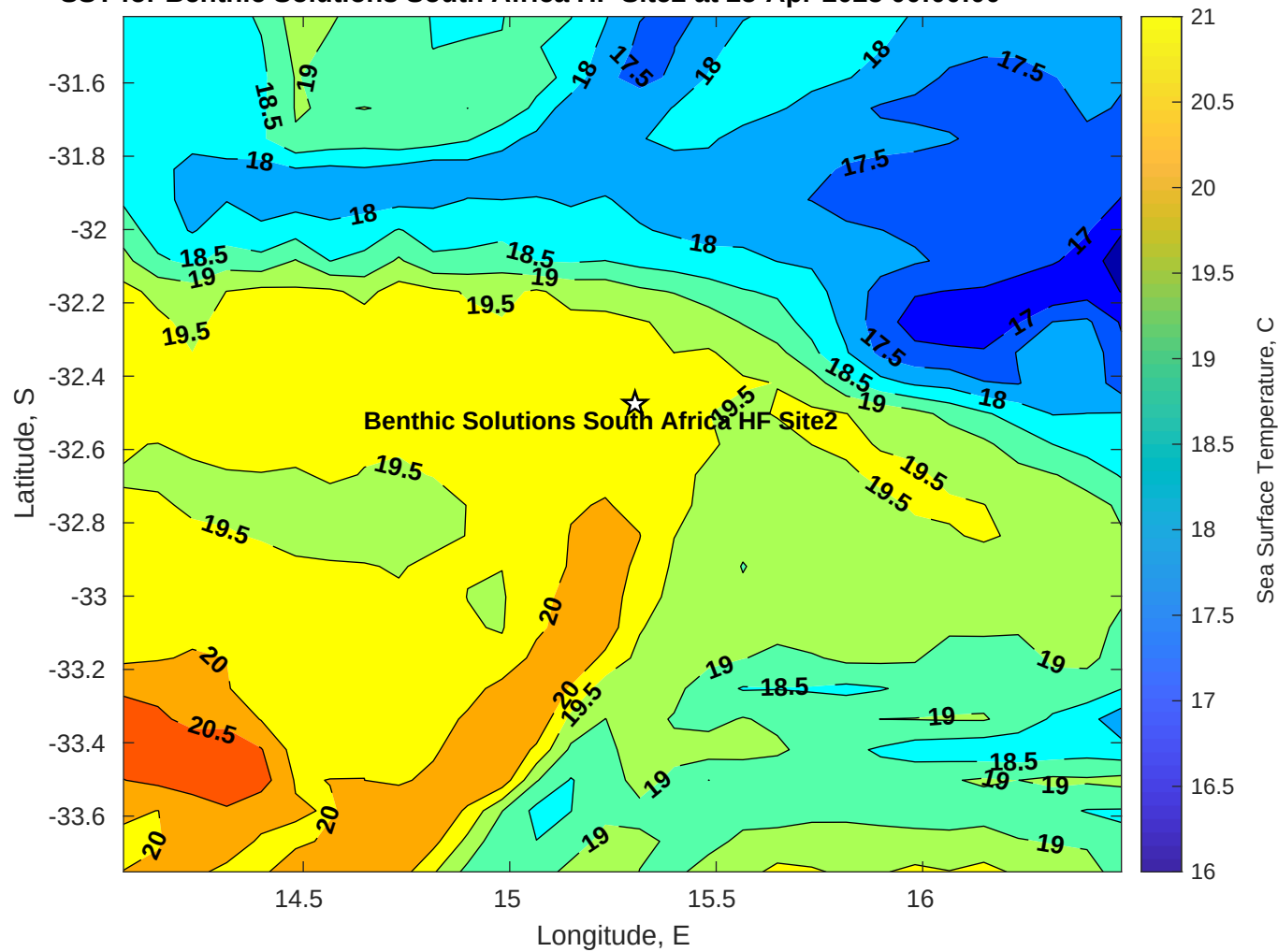
SST for Benthic Solutions South Africa HF Site2 at 25-Apr-2025 00:00:00
