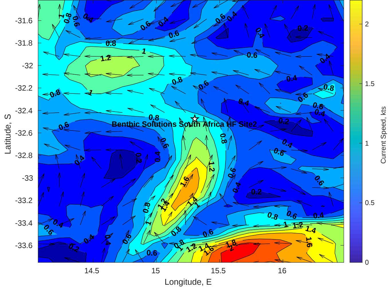
Surface Currents for Benthic Solutions South Africa HF Site2 at 25-Apr-2025 00:00:00
