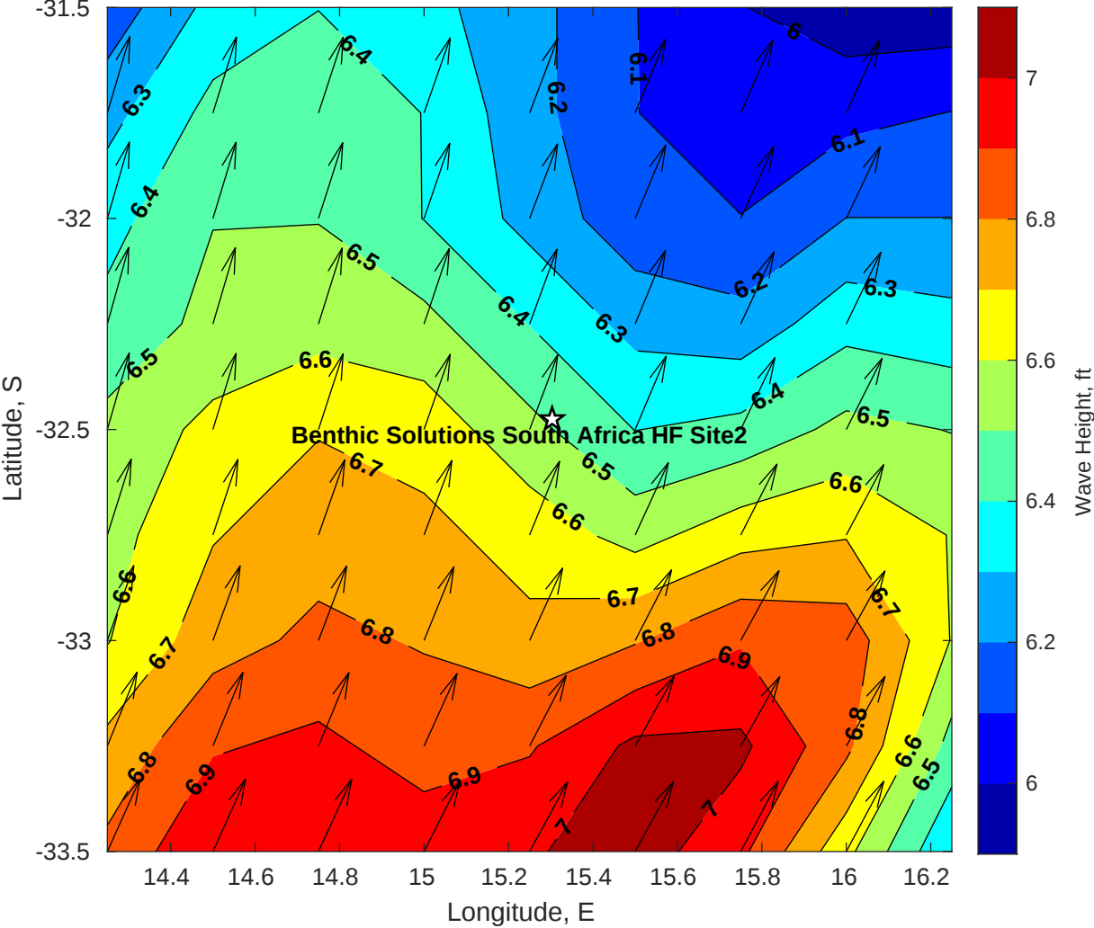
Wave Height (ft) for Benthic Solutions South Africa HF Site2 at 26-Apr-2025 09:00:00
