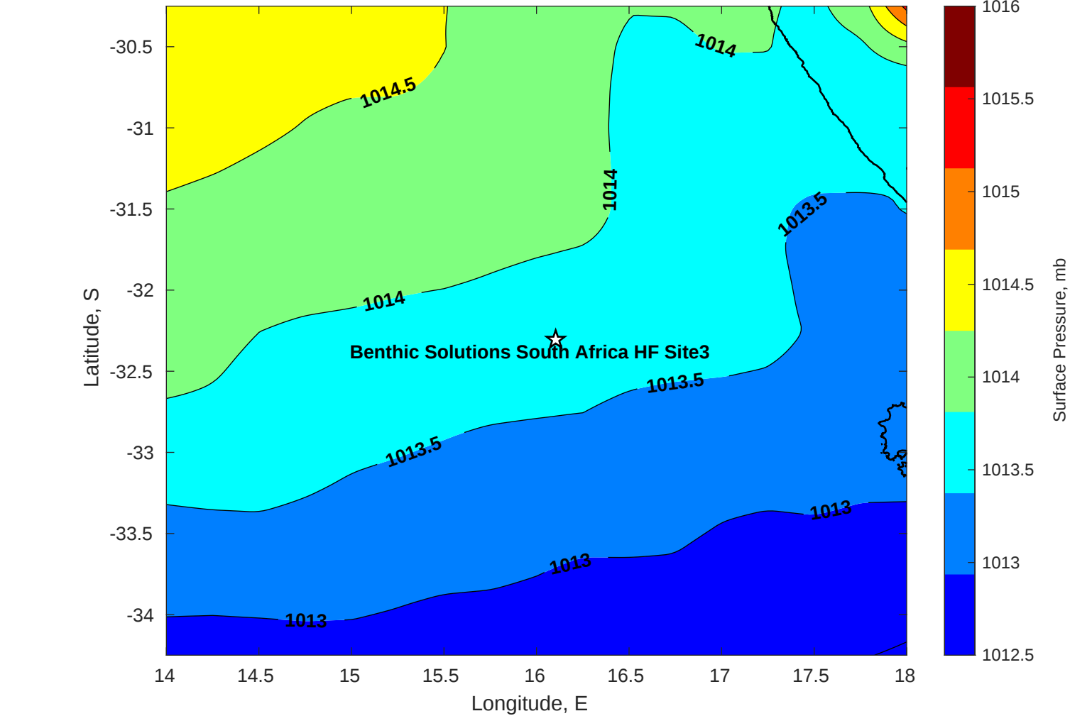
Surface Pressure (mb) for Benthic Solutions South Africa HF Site3 at 28-Apr-2025 00:00:00
