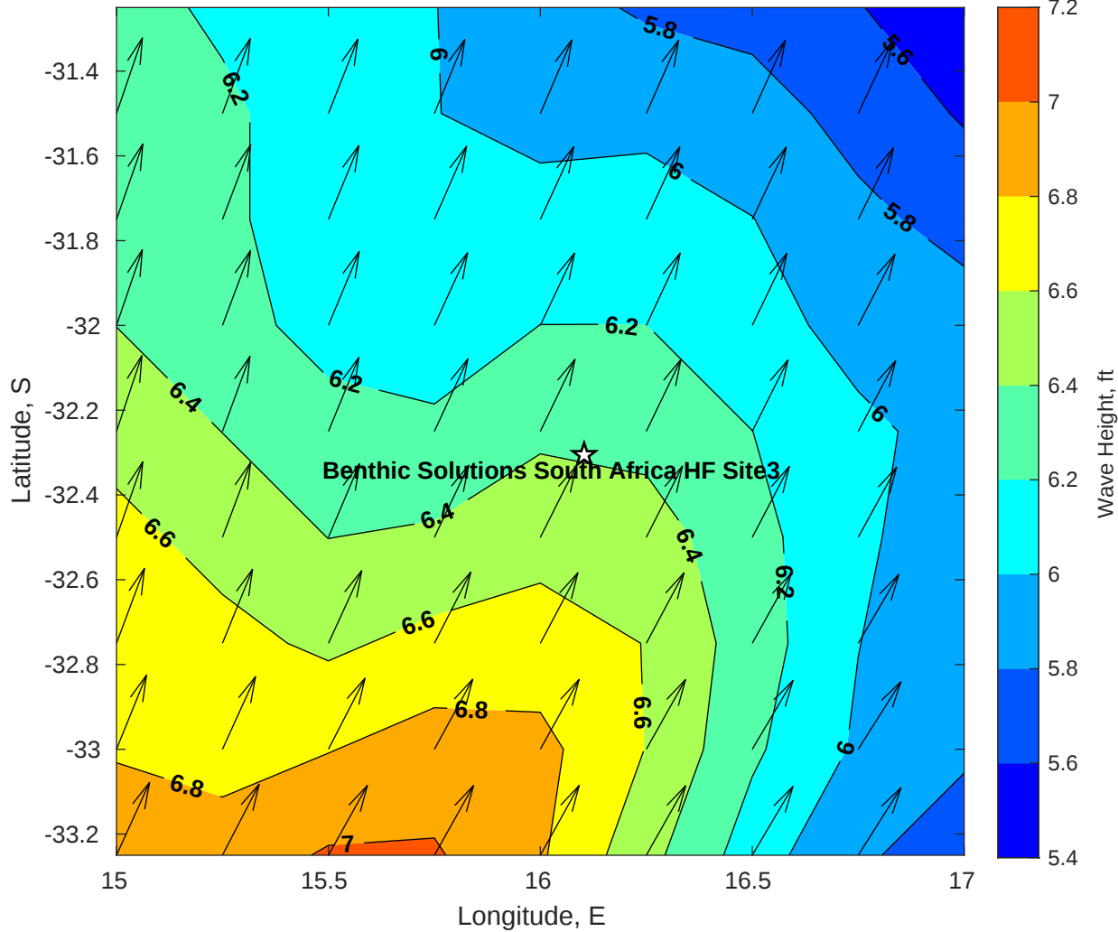
Wave Height (ft) for Benthic Solutions South Africa HF Site3 at 26-Apr-2025 09:00:00
