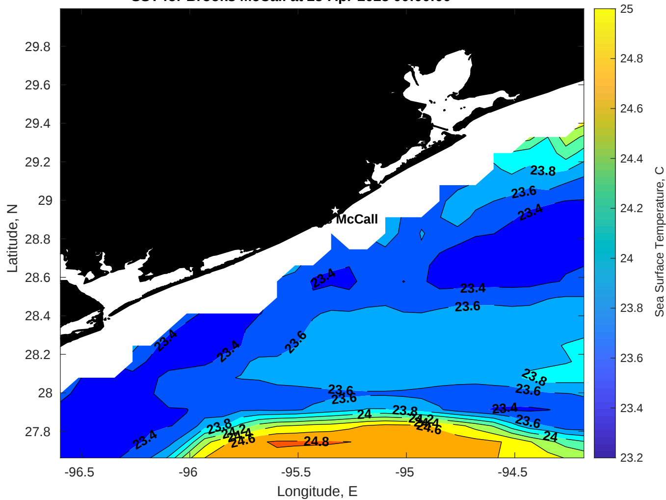
SST for Brooks McCall at 25-Apr-2025 00:00:00
