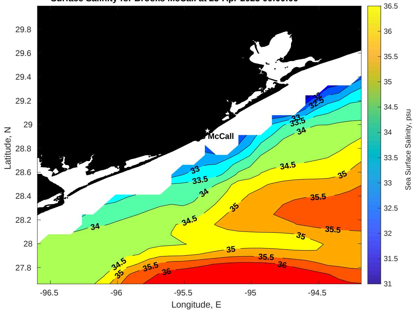
Surface Salinity for Brooks McCall at 25-Apr-2025 00:00:00
