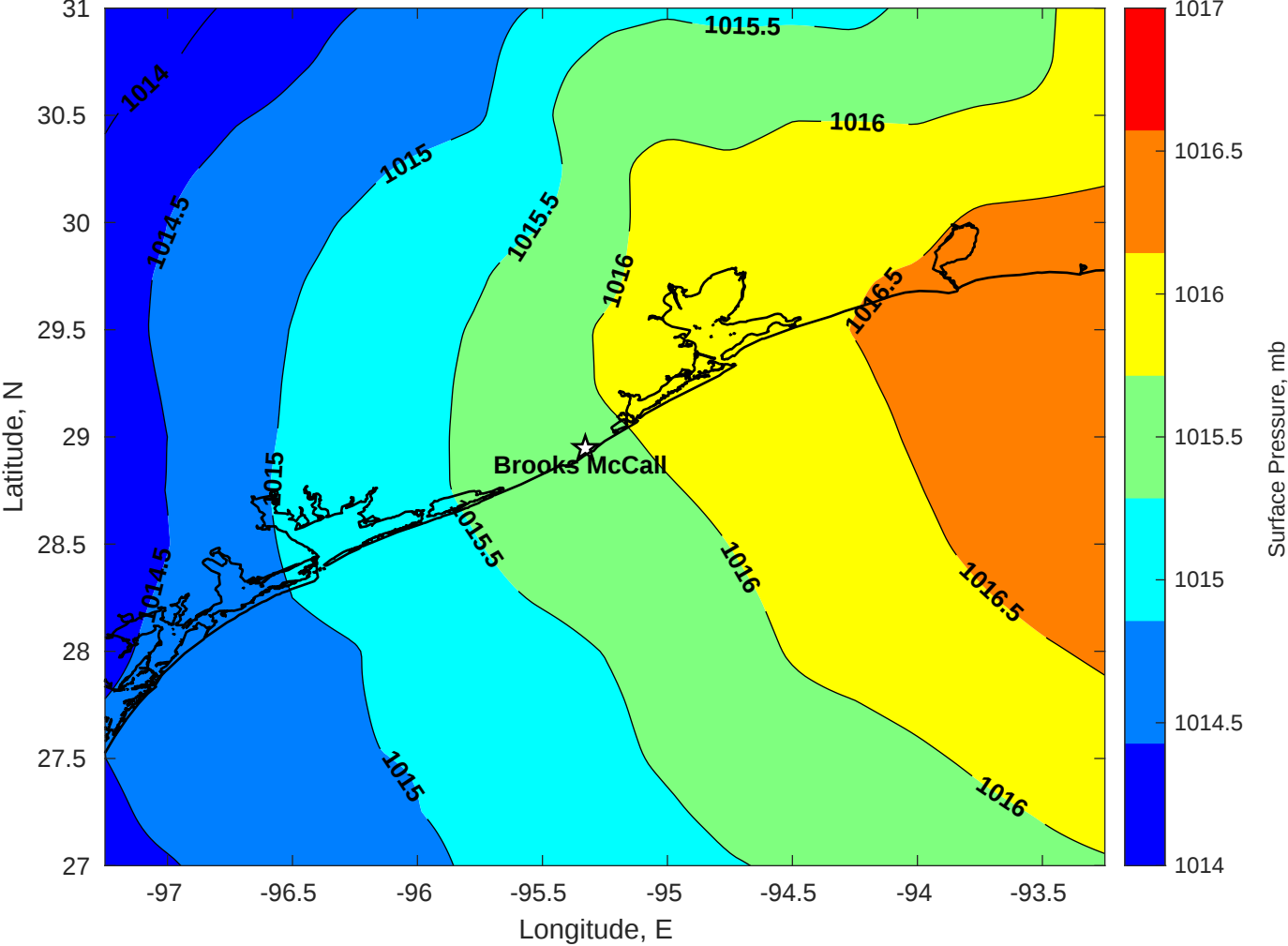
Surface Pressure (mb) for Brooks McCall at 27-Apr-2025 00:00:00
