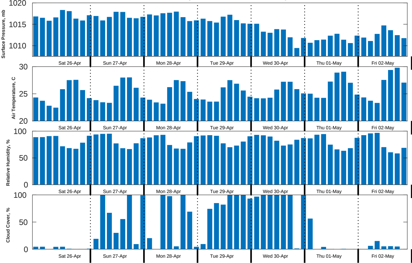
Met Forecast for Brooks McCall from 26-Apr-2025 00:00:00 to 03-May-2025 00:00:00
