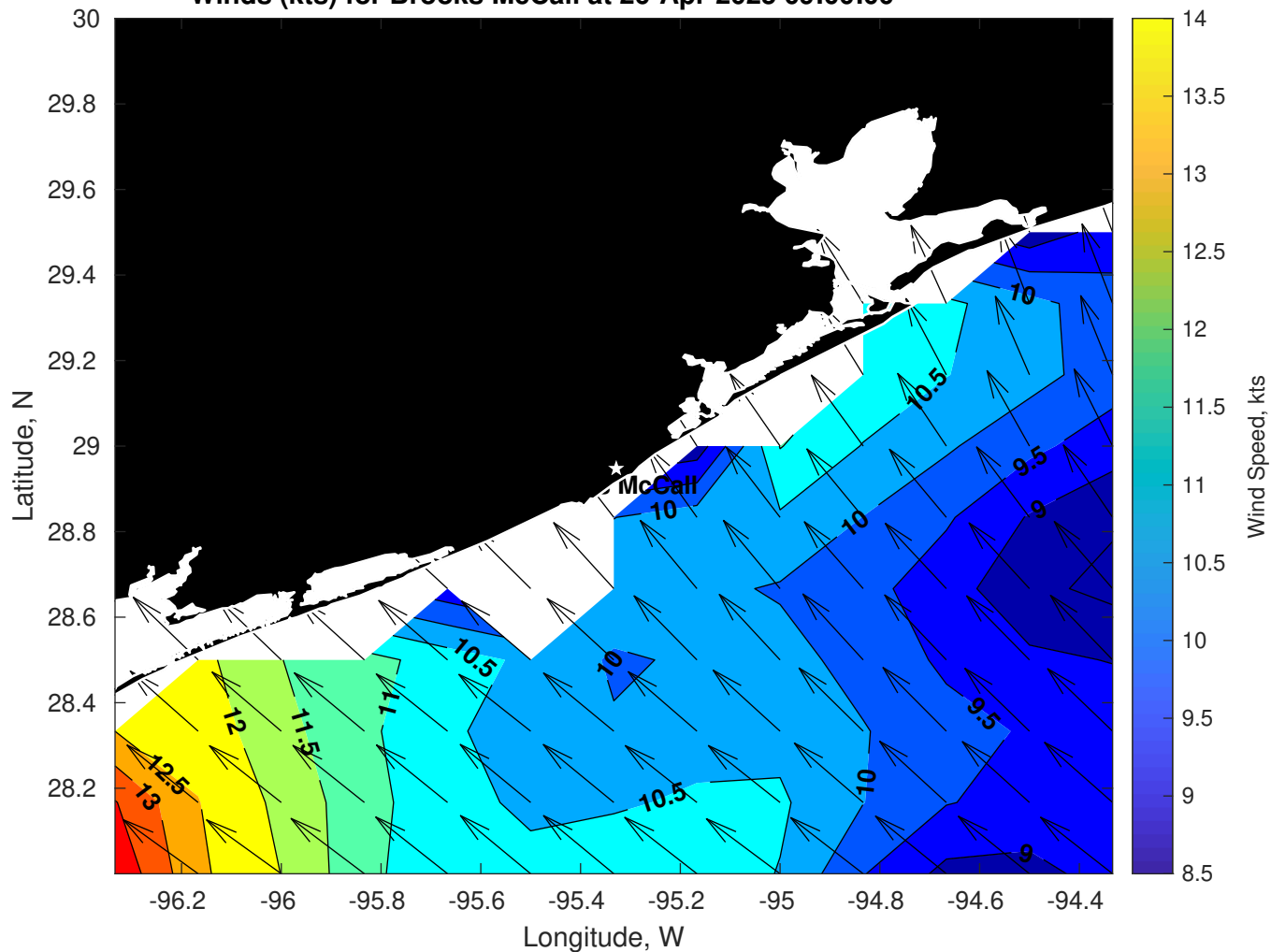
Winds (kts) for Brooks McCall at 26-Apr-2025 09:00:00
