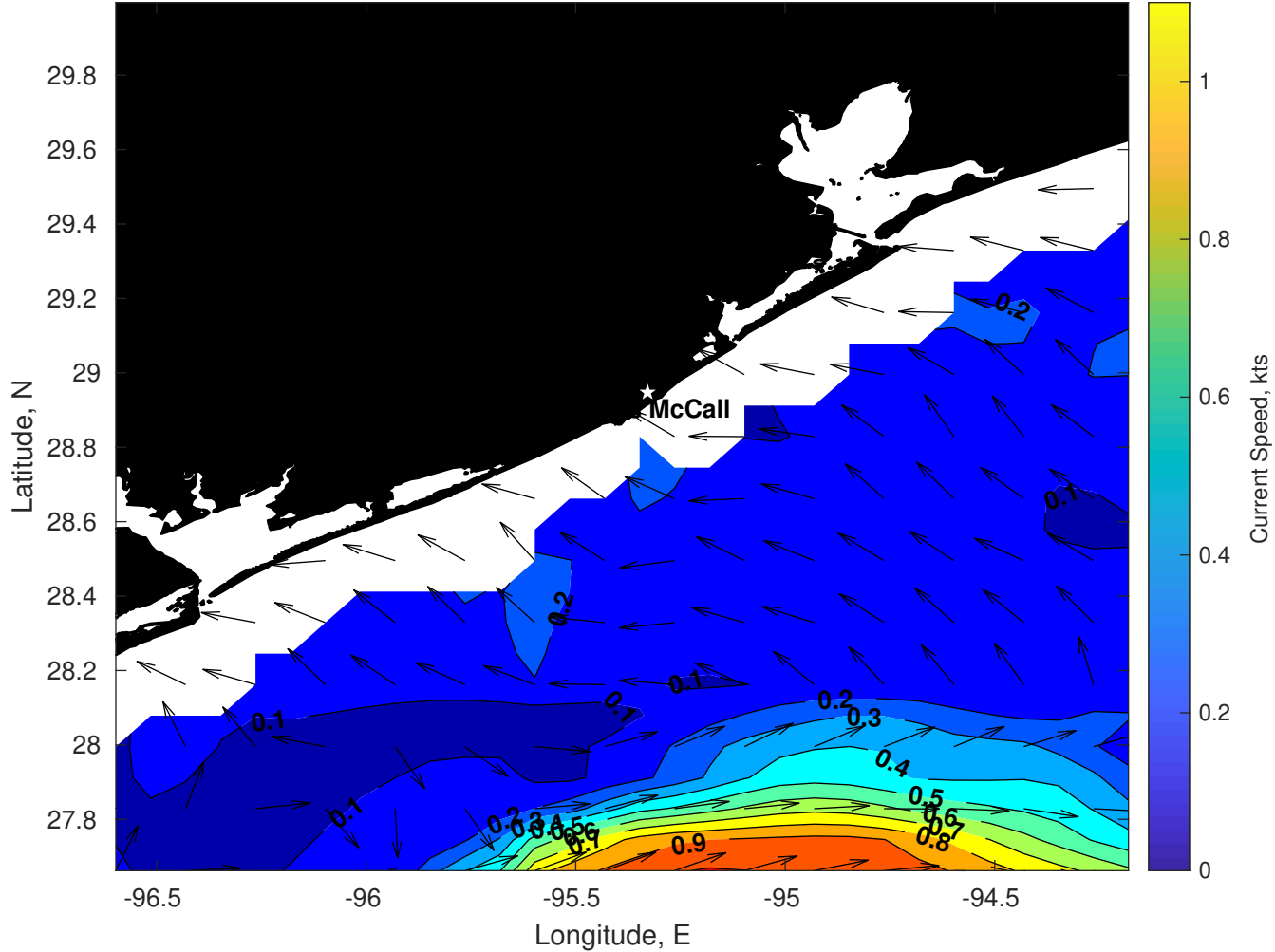
Surface Currents for Brooks McCall at 25-Apr-2025 00:00:00
