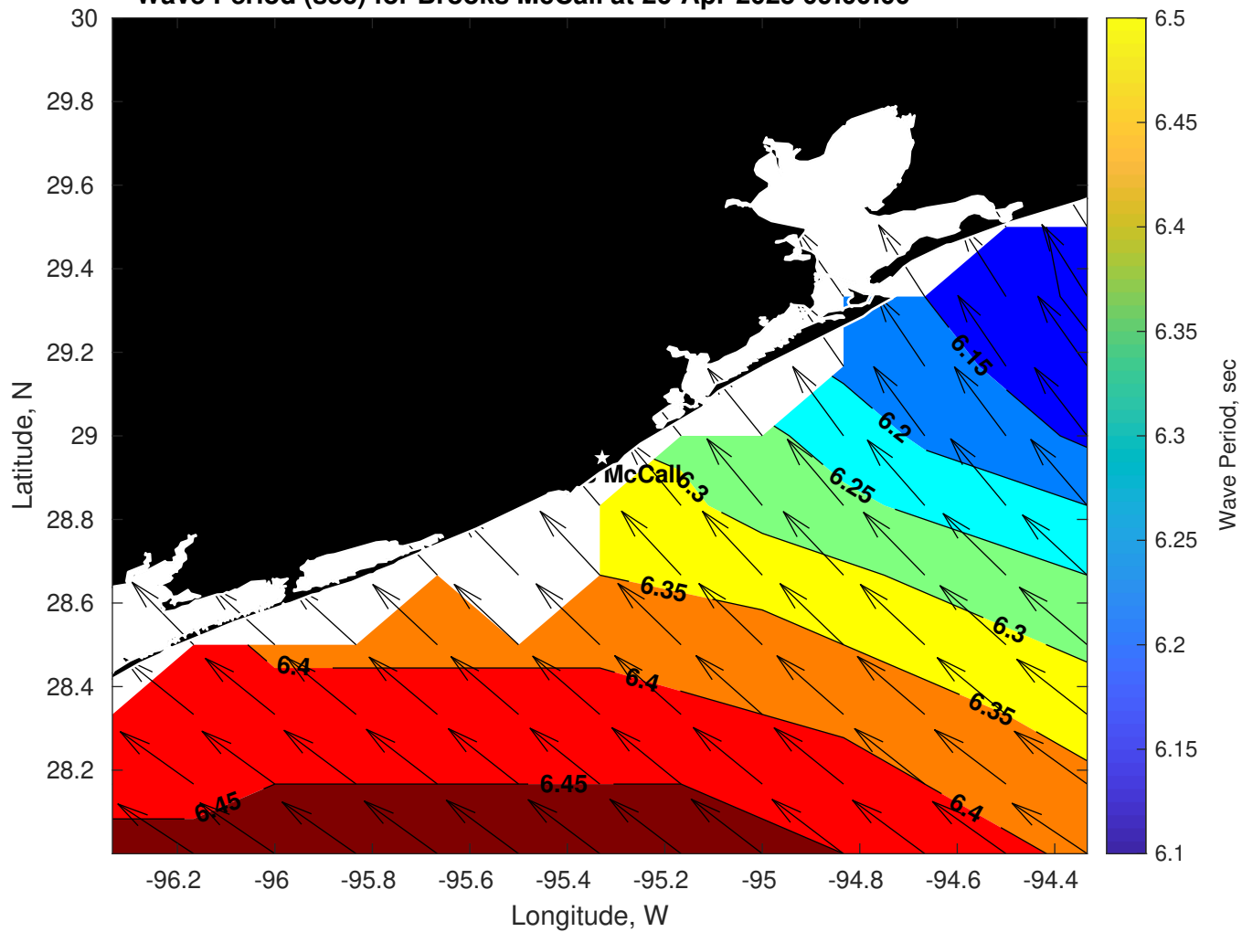
Wave Period (sec) for Brooks McCall at 26-Apr-2025 09:00:00
