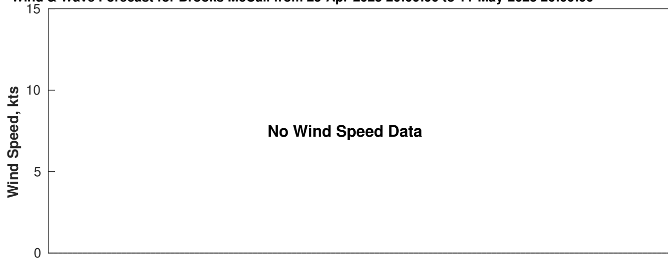
Wind & Wave Forecast for Brooks McCall from 25-Apr-2025 20:00:00 to 11-May-2025 20:00:00
