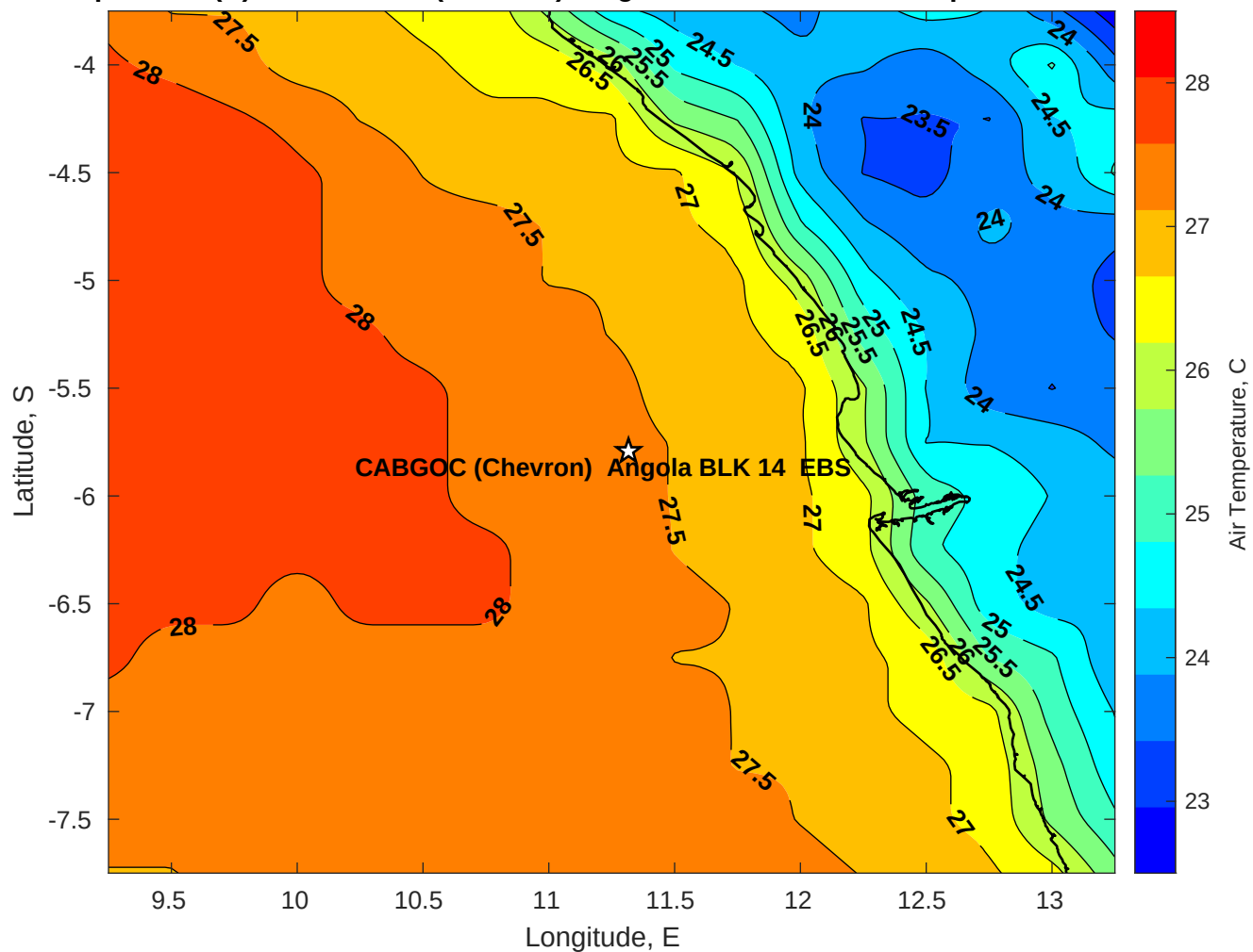
Air Temperature (C) for CABGOC (Chevron) Angola BLK 14 EBS at 26-Apr-2025
