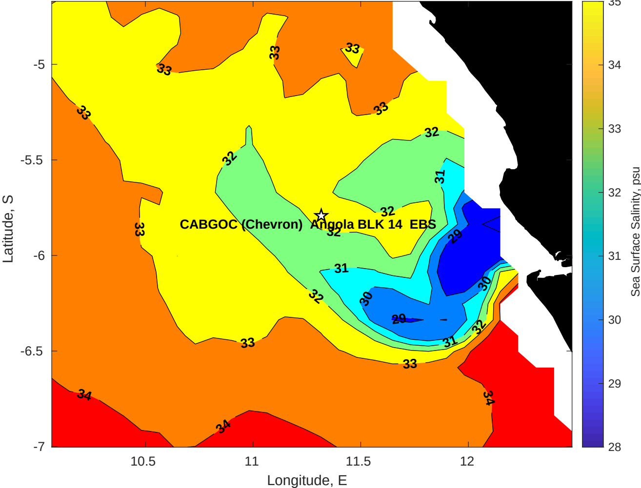
Surface Salinity for CABGOC (Chevron) Angola BLK 14 EBS at 25-Apr-2025 00:00:00
