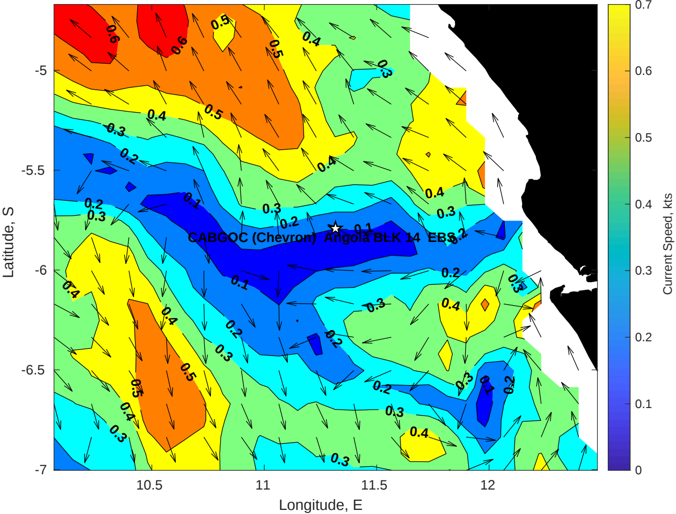
Surface Currents for CABGOC (Chevron) Angola BLK 14 EBS at 25-Apr-2025 00:00:00
