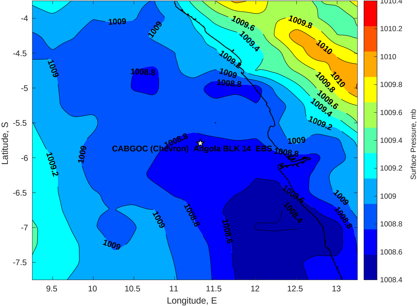
Surface Pressure (mb) for CABGOC (Chevron) Angola BLK 14 EBS at 28-Apr-2025 00:00:00
