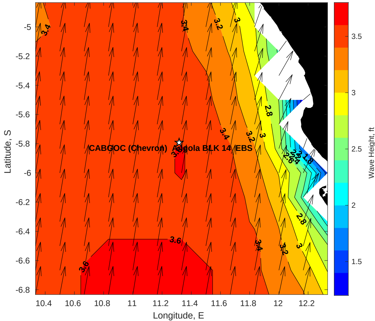
Wave Height (ft) for CABGOC (Chevron) Angola BLK 14 EBS at 26-Apr-2025 09:00:00
