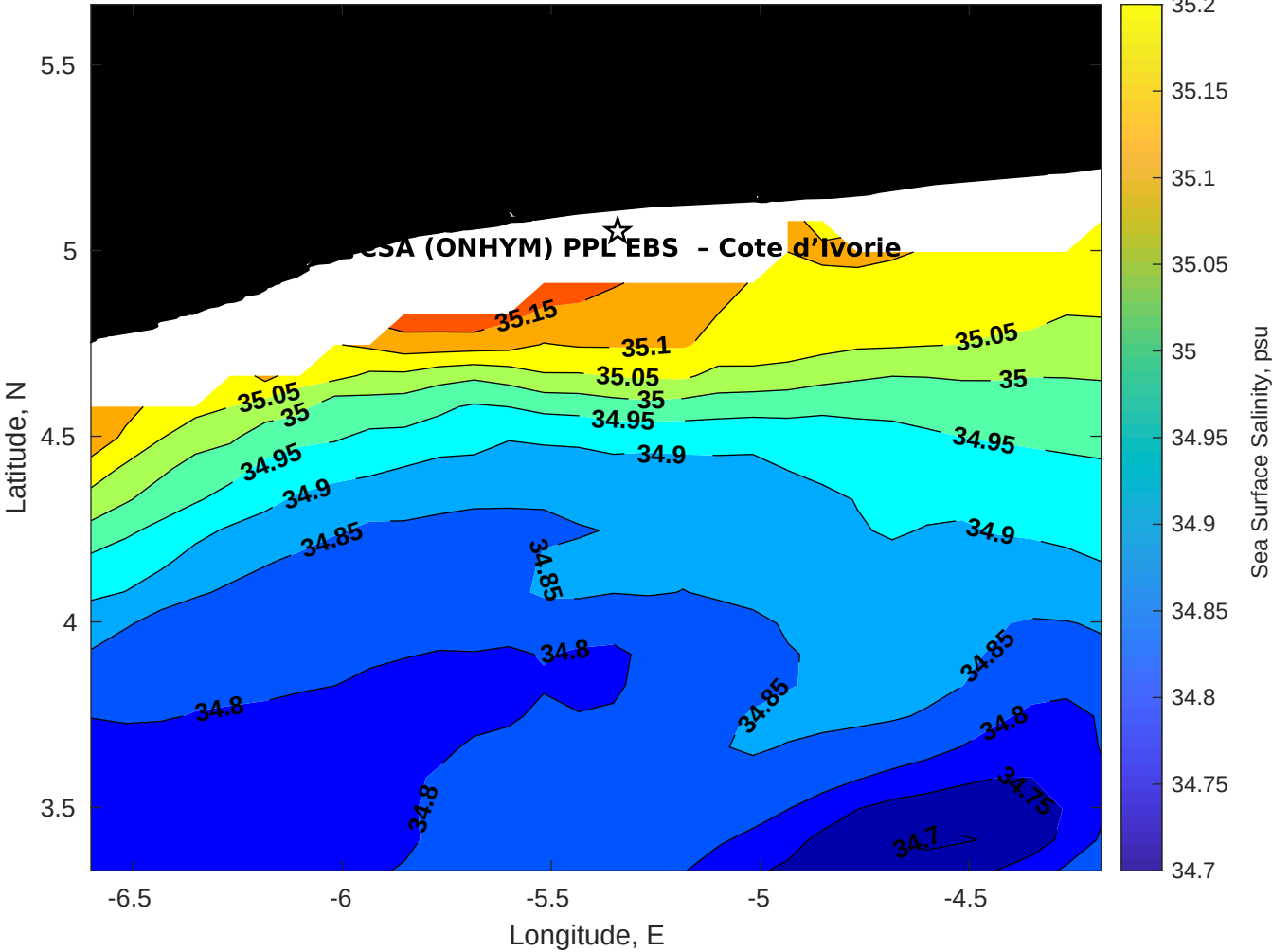
Surface Salinity for CSA (ONHYM) PPL EBS - Cote d'Ivoire at 25-Apr-2025 00:00:00
