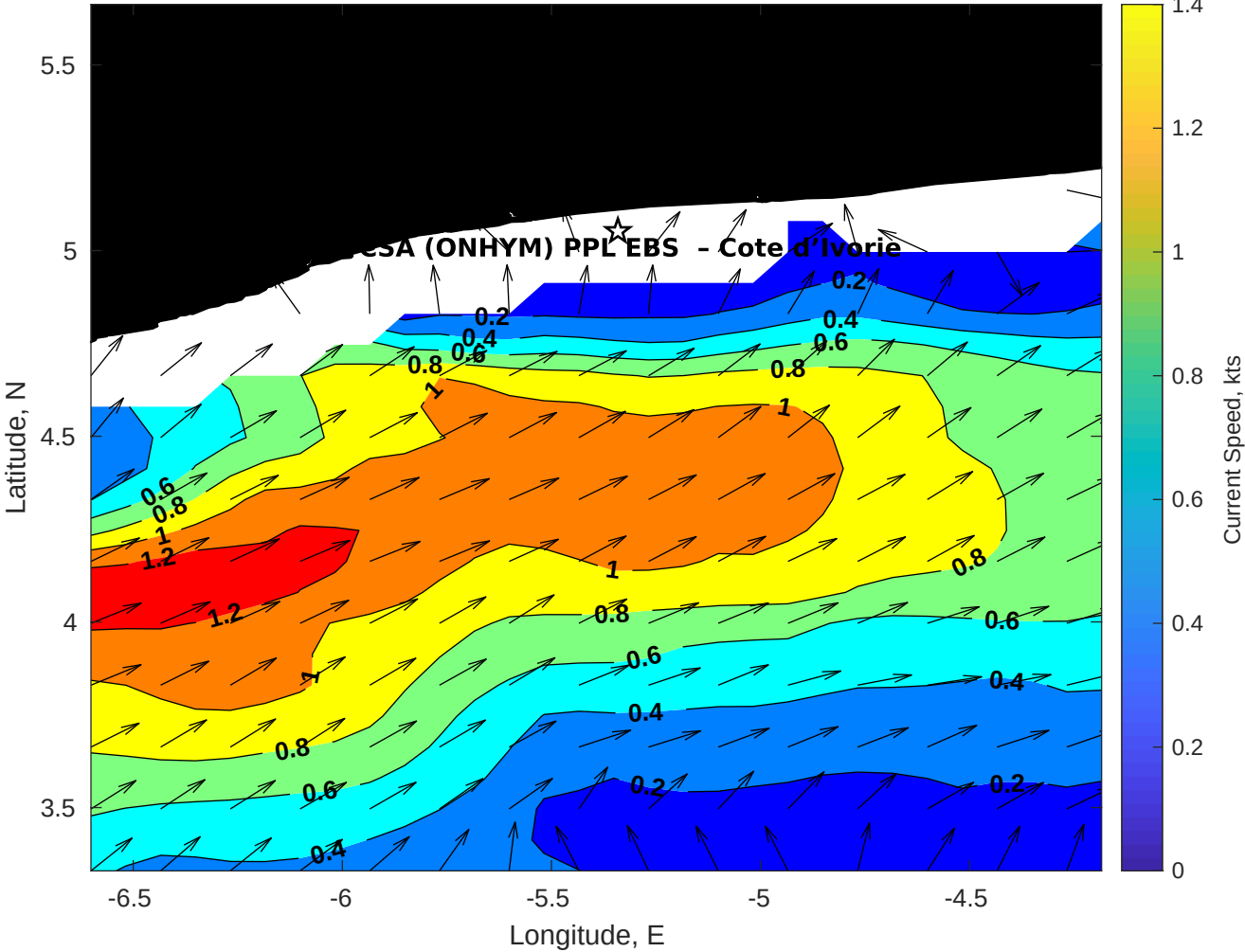
Surface Currents for CSA (ONHYM) PPL EBS - Cote d'Ivoire at 25-Apr-2025 00:00:00
