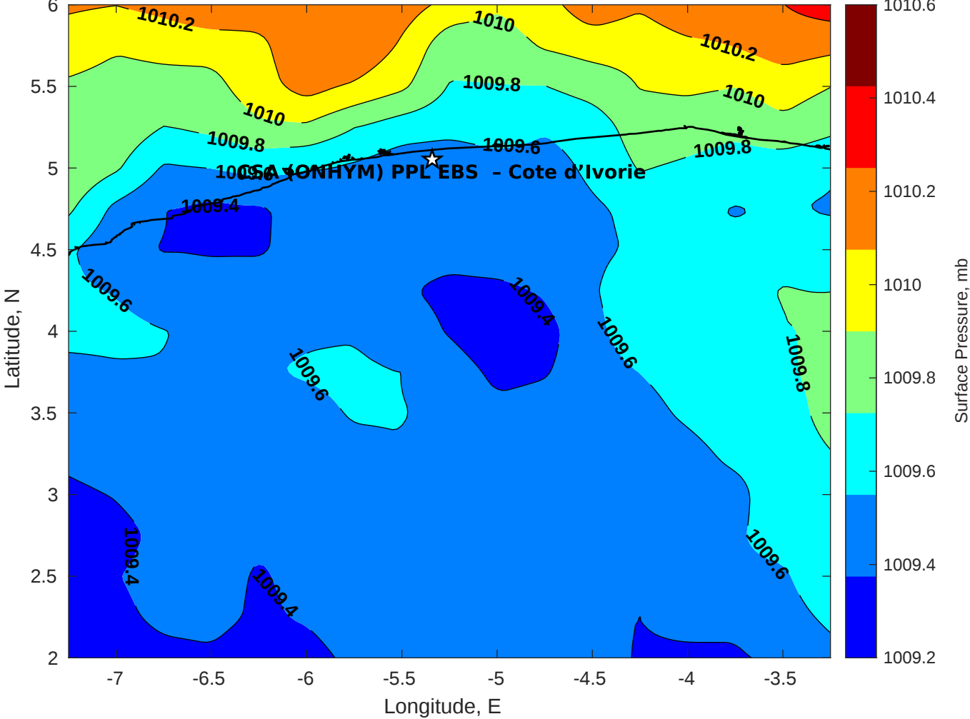
Surface Pressure (mb) for CSA (ONHYM) PPL EBS - Cote d'Ivoire at 28-Apr-2025 00:00:00
