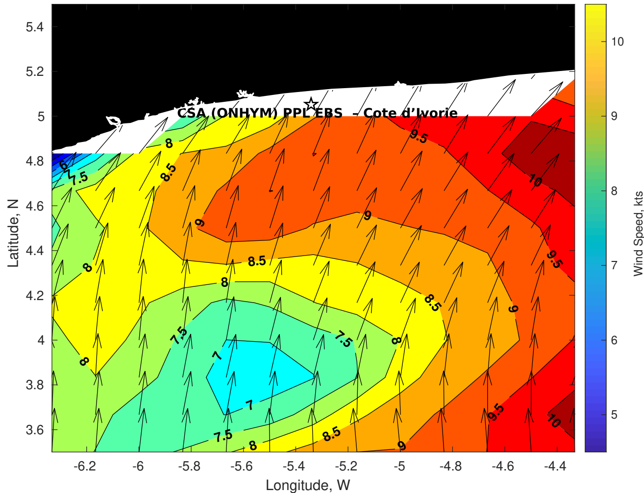
Winds (kts) for CSA (ONHYM) PPL EBS - Cote d'Ivoire at 26-Apr-2025 09:00:00
