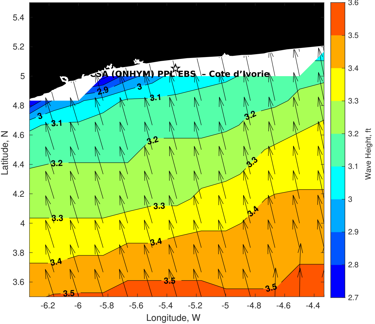
Wave Height (ft) for CSA (ONHYM) PPL EBS - Cote d'Ivoire at 26-Apr-2025 09:00:00
