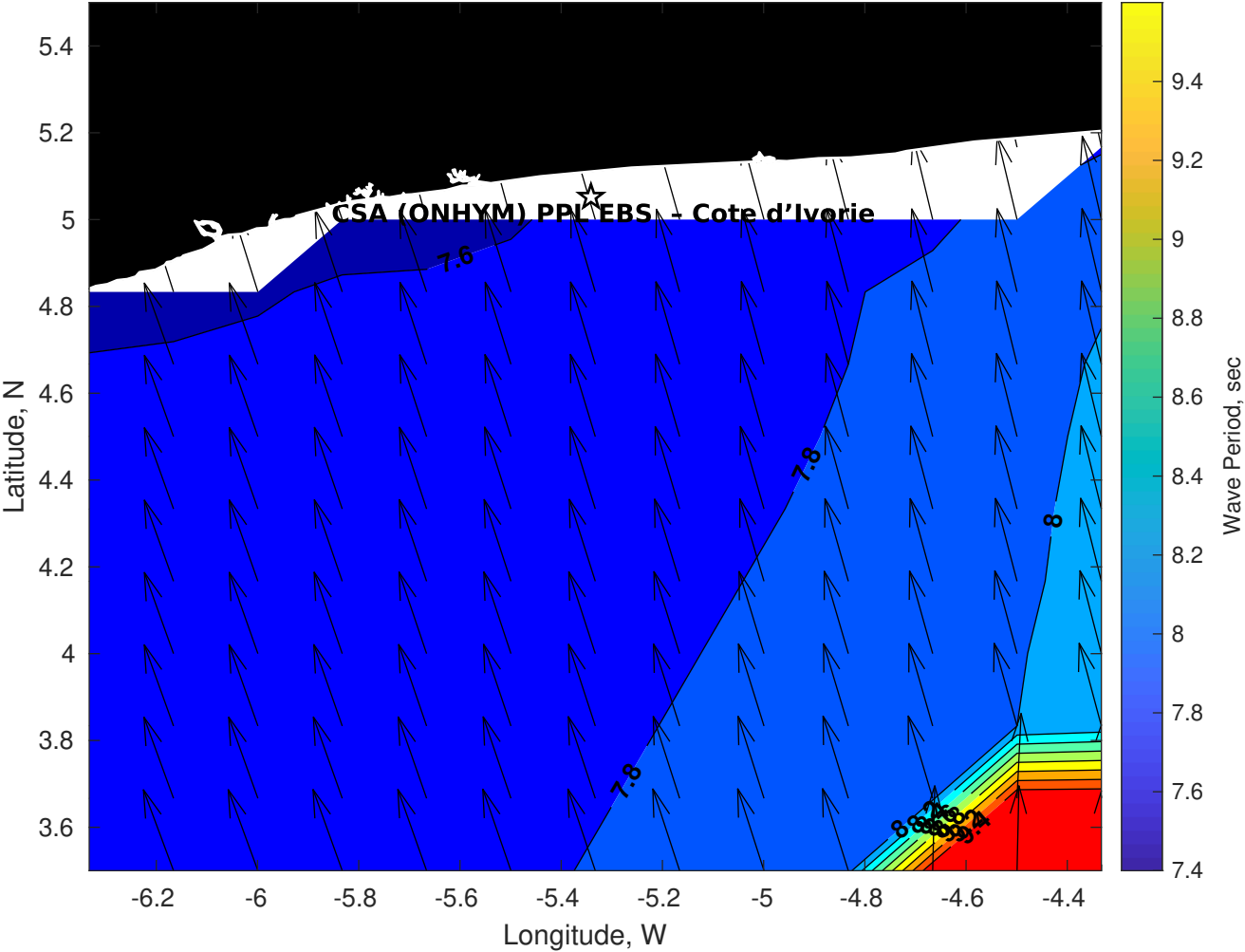
Wave Period (sec) for CSA (ONHYM) PPL EBS - Cote d'Ivoire at 26-Apr-2025 09:00:00
