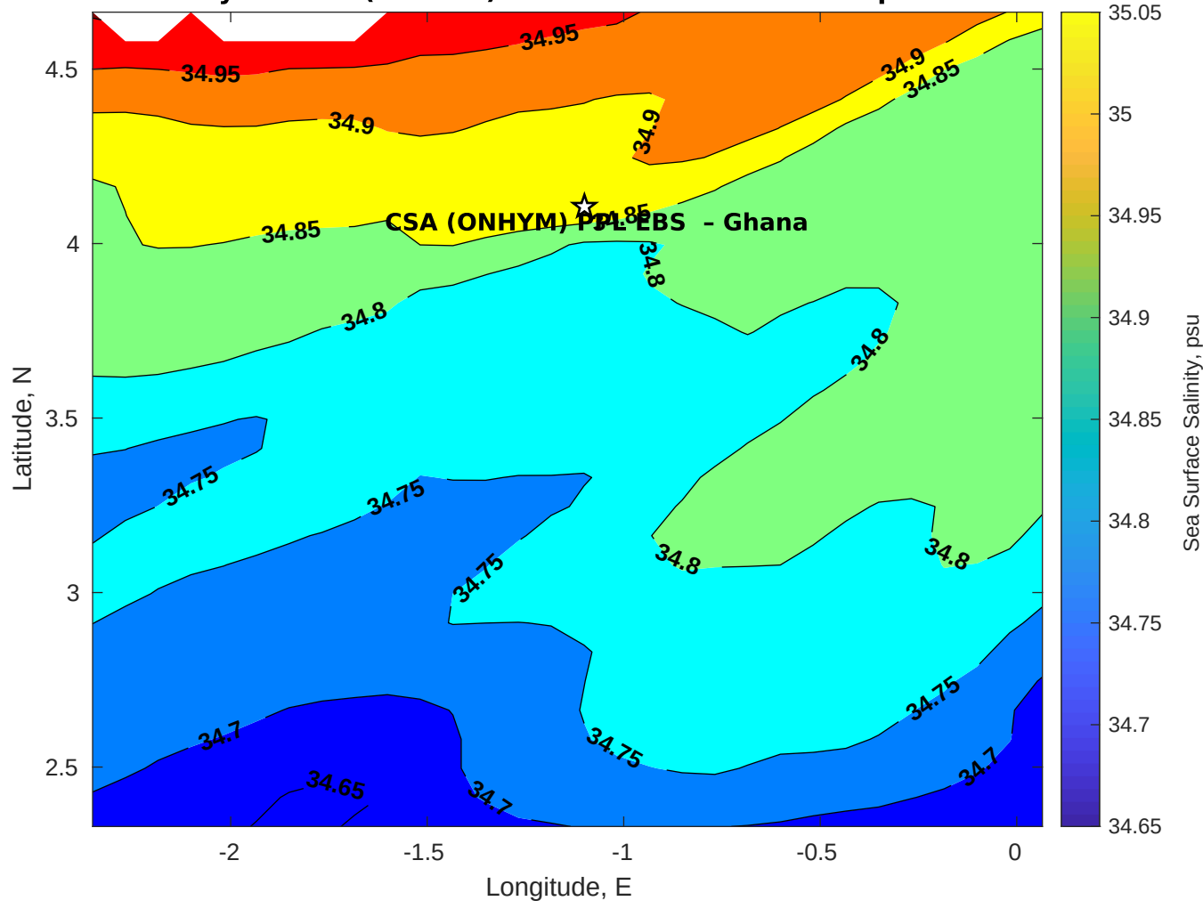
Surface Salinity for CSA (ONHYM) PPL EBS - Ghana at 25-Apr-2025 00:00:00
