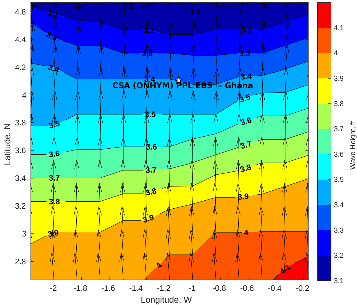
Wave Height (ft) for CSA (ONHYM) PPL EBS - Ghana at 26-Apr-2025 09:00:00
