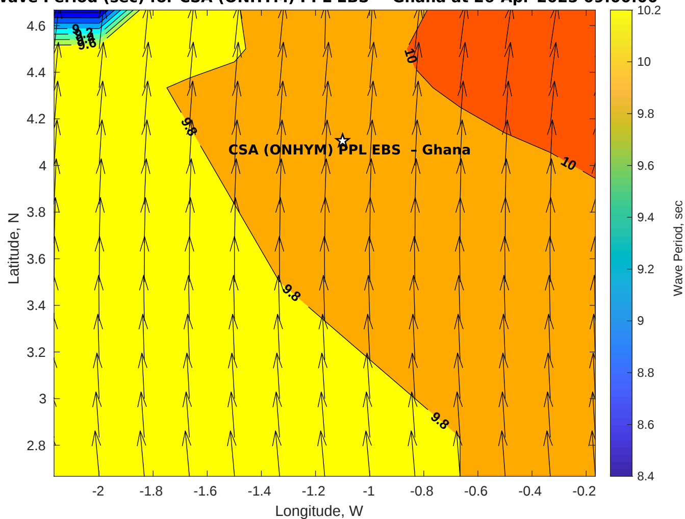
Wave Period (sec) for CSA (ONHYM) PPL EBS - Ghana at 26-Apr-2025 09:00:00
