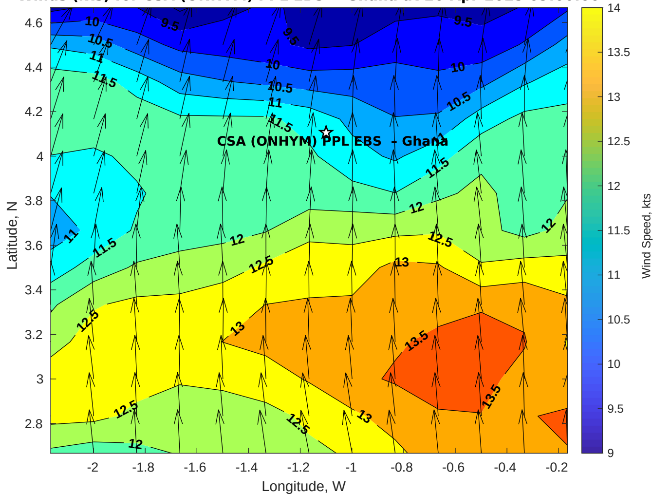
Winds (kts) for CSA (ONHYM) PPL EBS - Ghana at 26-Apr-2025 09:00:00
