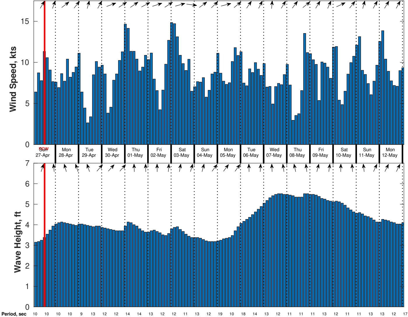
Wind & Wave Forecast for CSA (ONHYM) PPL EBS - Ghana from 26-Apr-2025 02:00:00 to 12-May-2025 02:00:00
