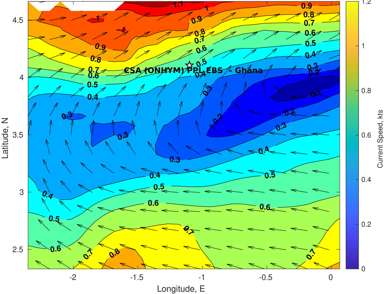
Surface Currents for CSA (ONHYM) PPL EBS - Ghana at 25-Apr-2025 00:00:00
