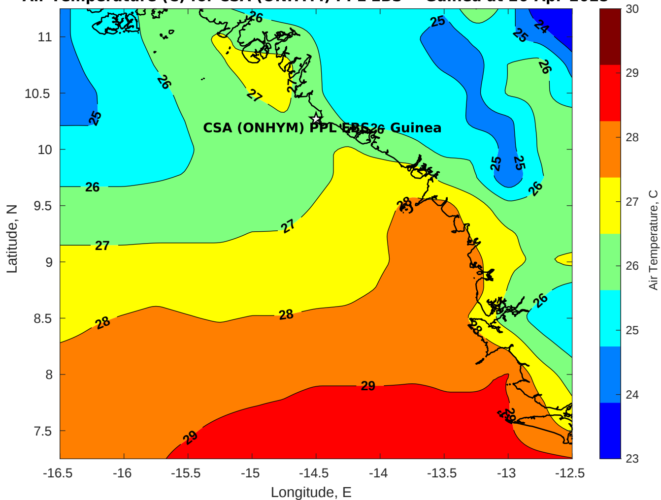
Air Temperature (C) for CSA (ONHYM) PPL EBS - Guinea at 26-Apr-2025
