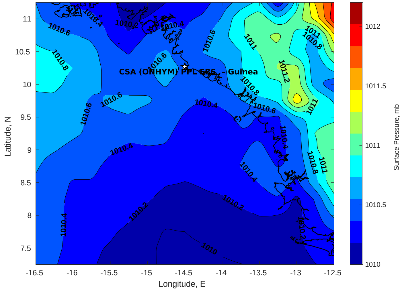
Surface Pressure (mb) for CSA (ONHYM) PPL EBS - Guinea at 28-Apr-2025 00:00:00
