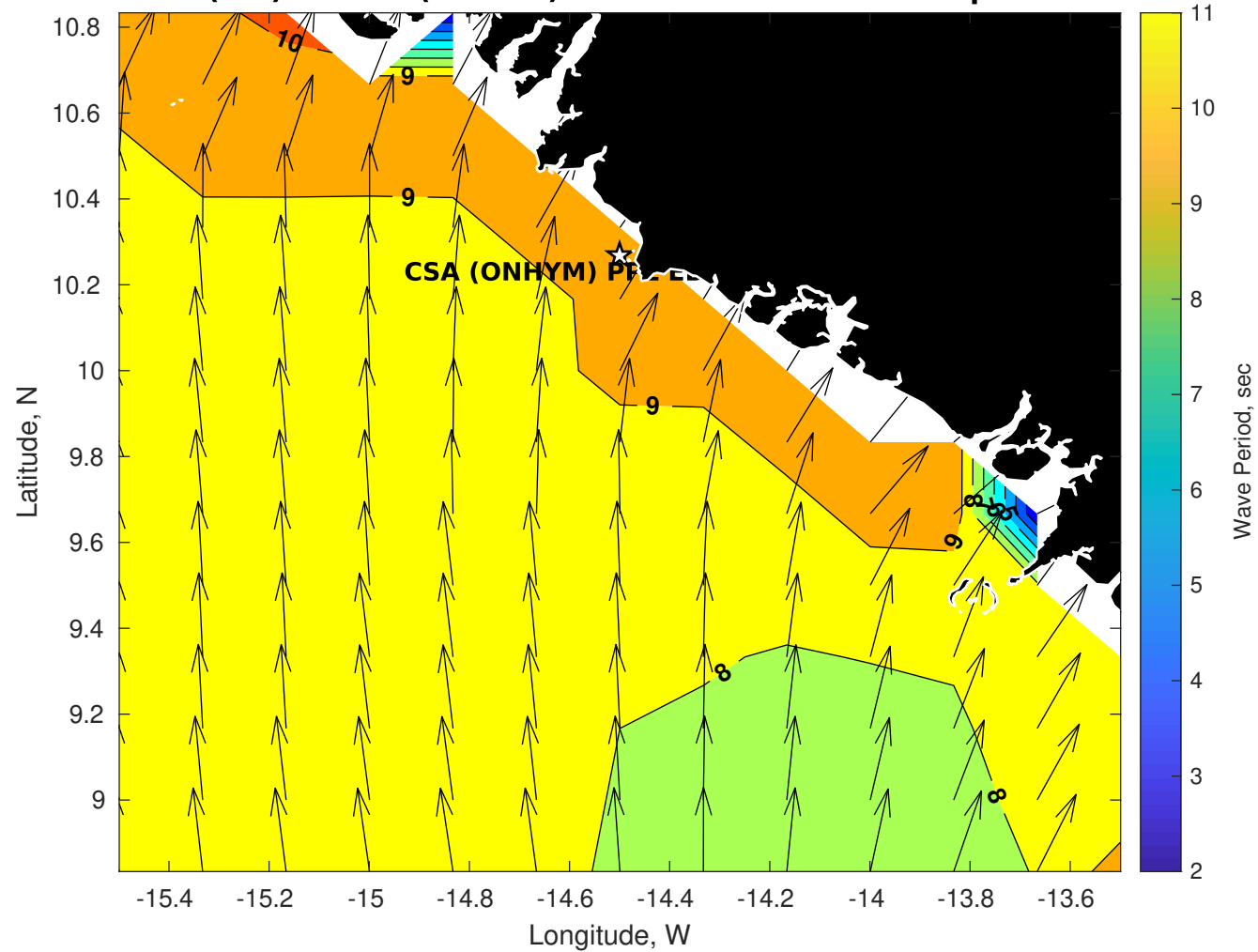
Wave Period (sec) for CSA (ONHYM) PPL EBS - Guinea at 26-Apr-2025 09:00:00
