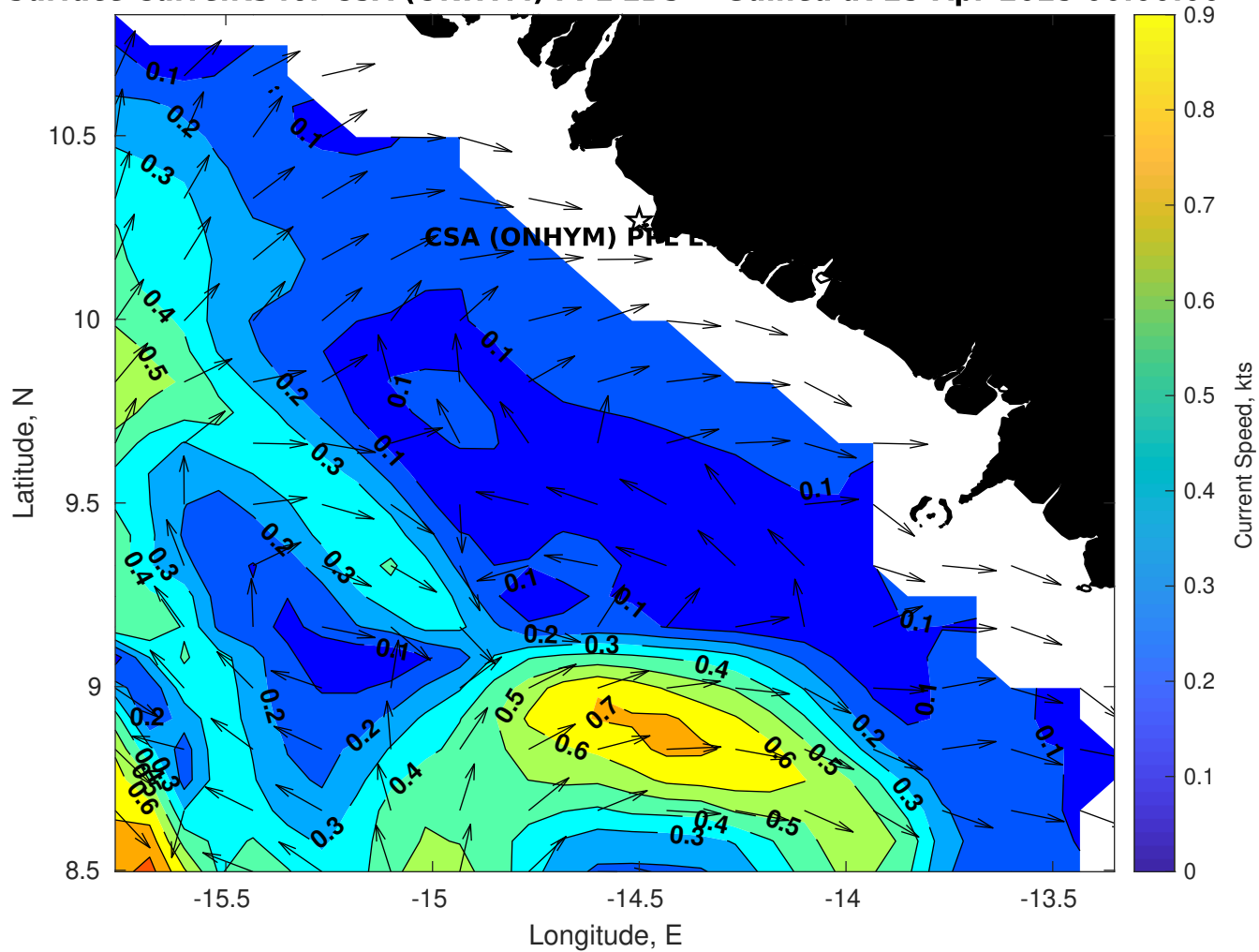
Surface Currents for CSA (ONHYM) PPL EBS - Guinea at 25-Apr-2025 00:00:00
