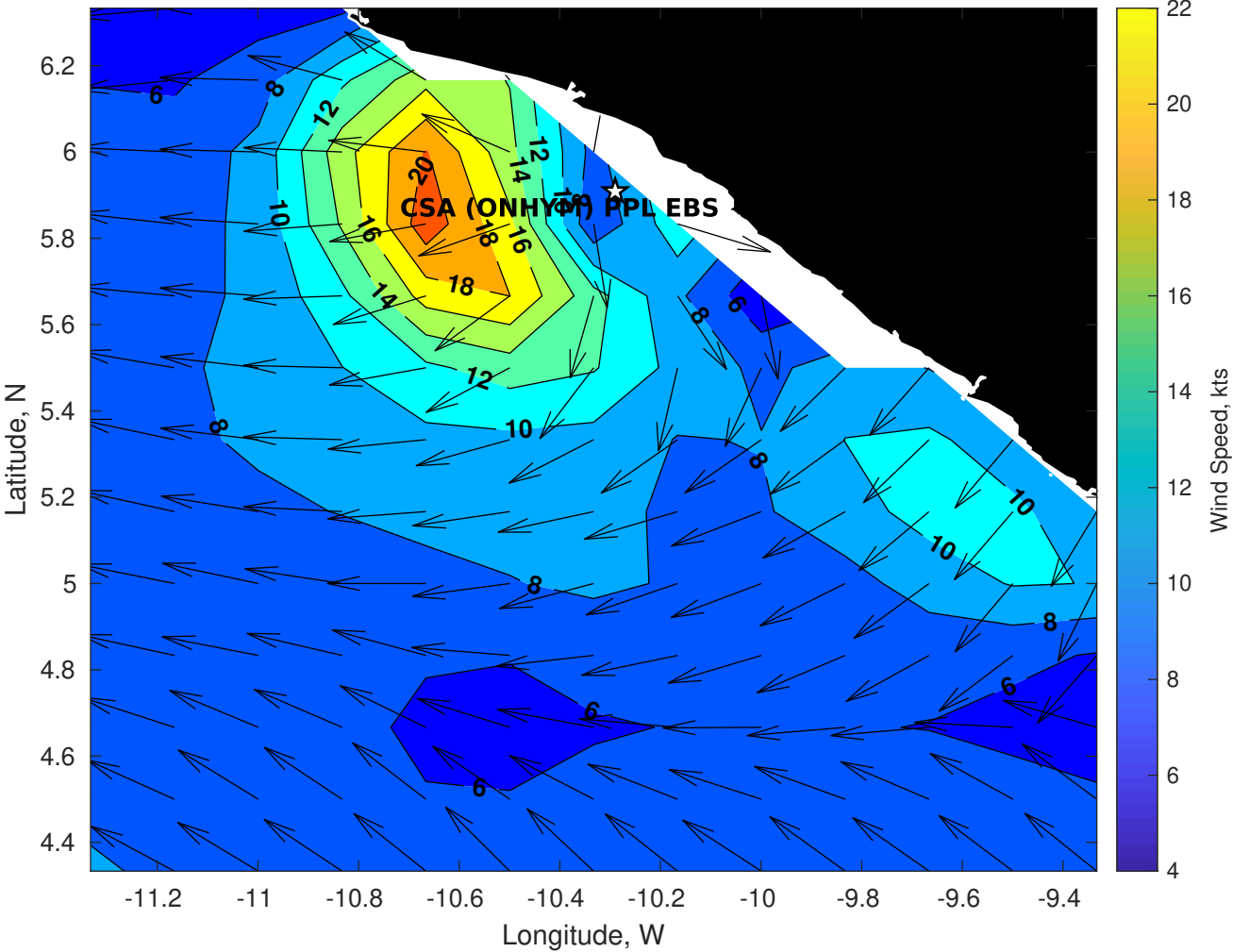
Winds (kts) for CSA (ONHYM) PPL EBS - Liberia at 26-Apr-2025 09:00:00
