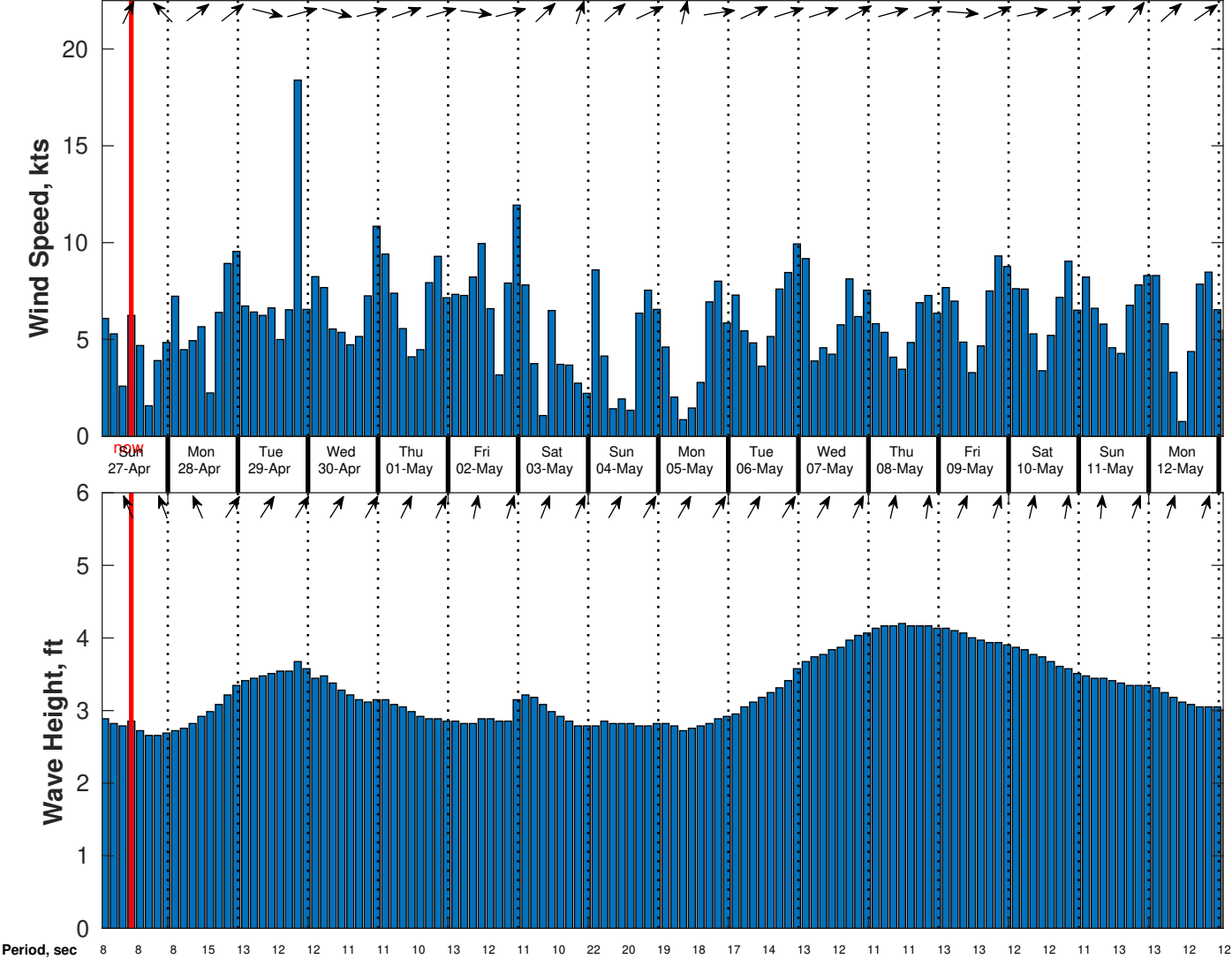
Wind & Wave Forecast for CSA (ONHYM) PPL EBS - Liberia from 26-Apr-2025 01:00:00 to 12-May-2025 01:00:00
