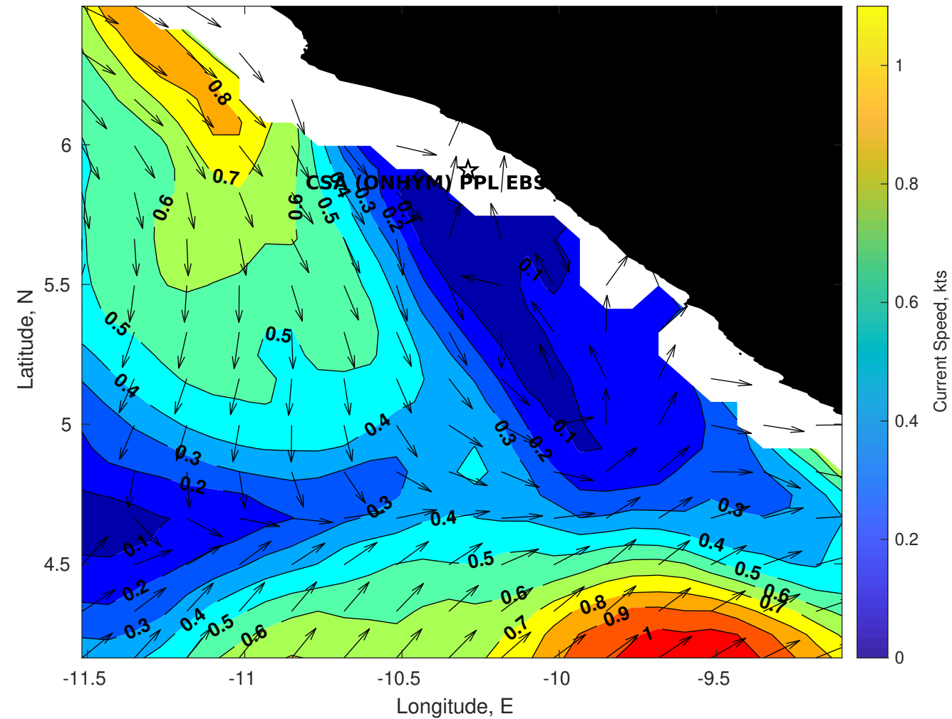
Surface Currents for CSA (ONHYM) PPL EBS - Liberia at 25-Apr-2025 00:00:00
