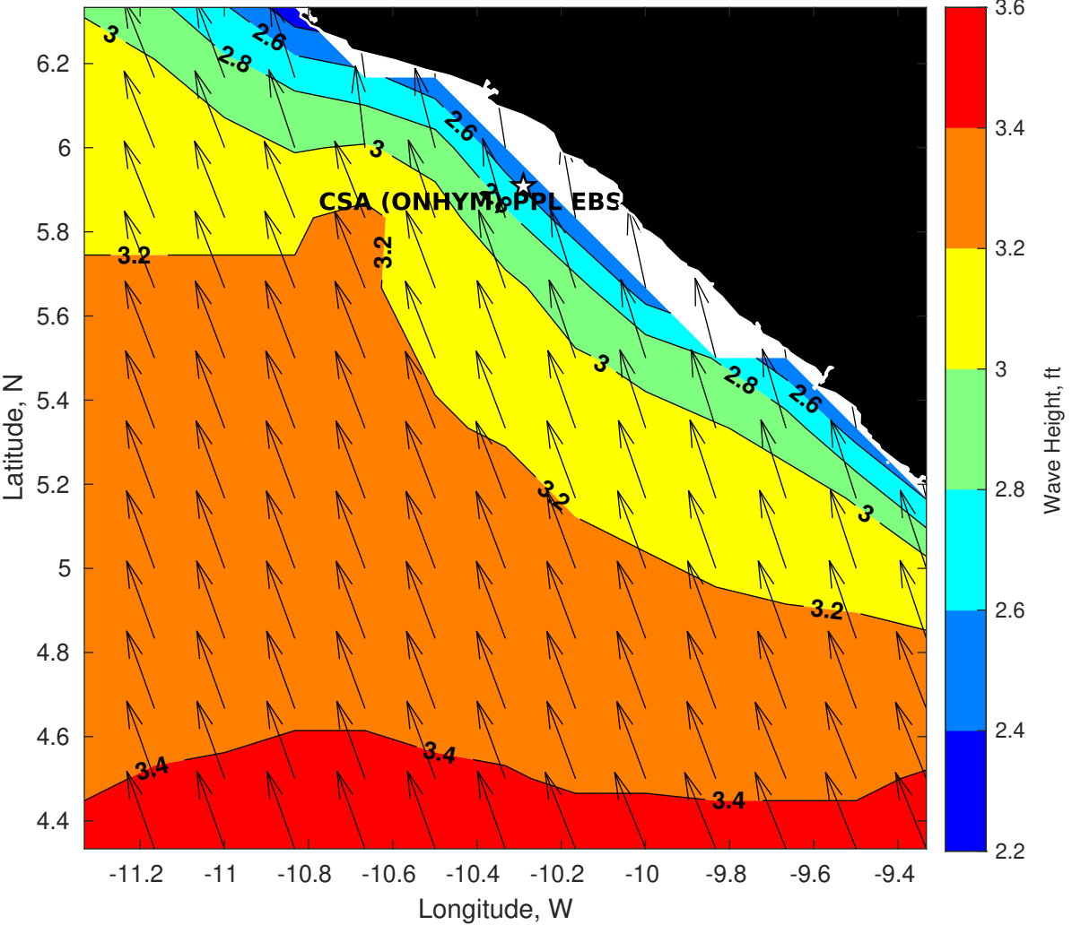
Wave Height (ft) for CSA (ONHYM) PPL EBS - Liberia at 26-Apr-2025 09:00:00
