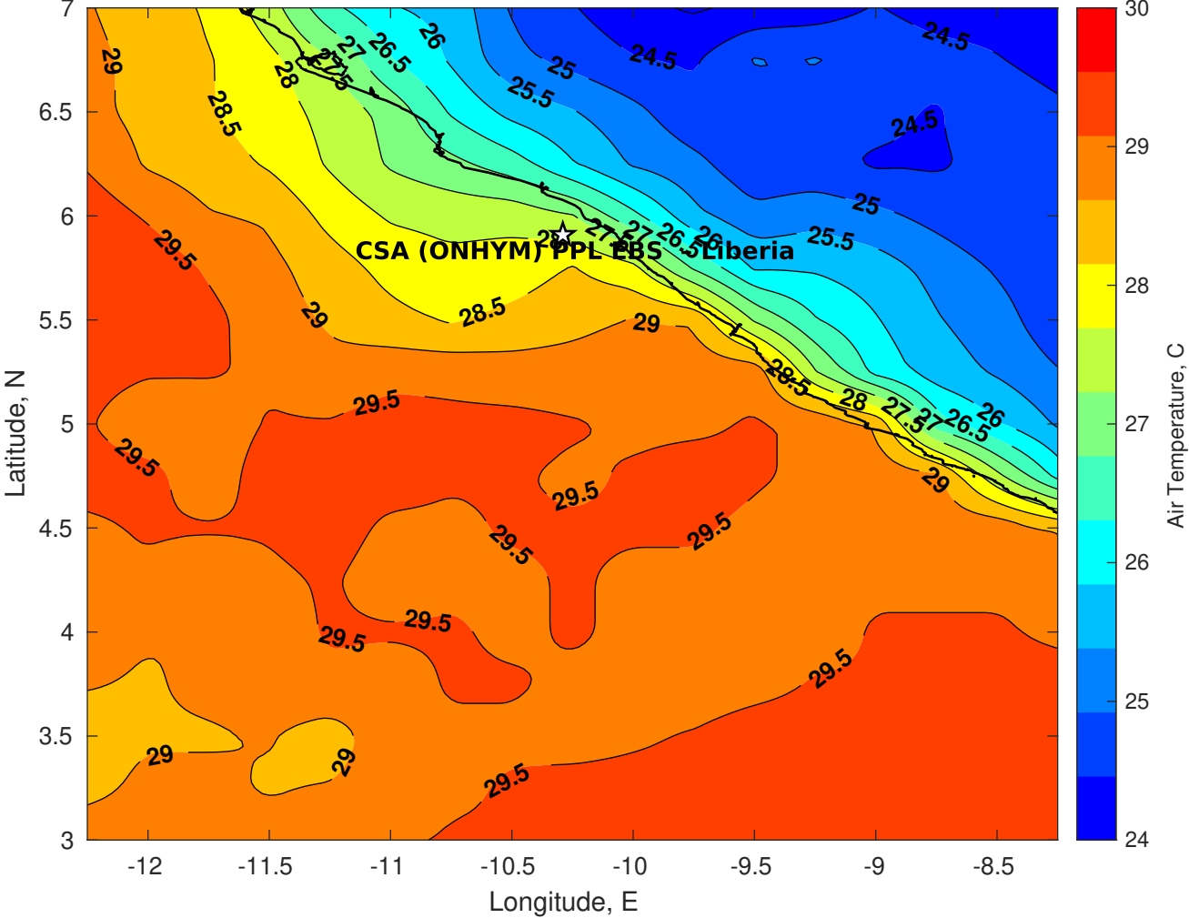
Air Temperature (C) for CSA (ONHYM) PPL EBS - Liberia at 26-Apr-2025
