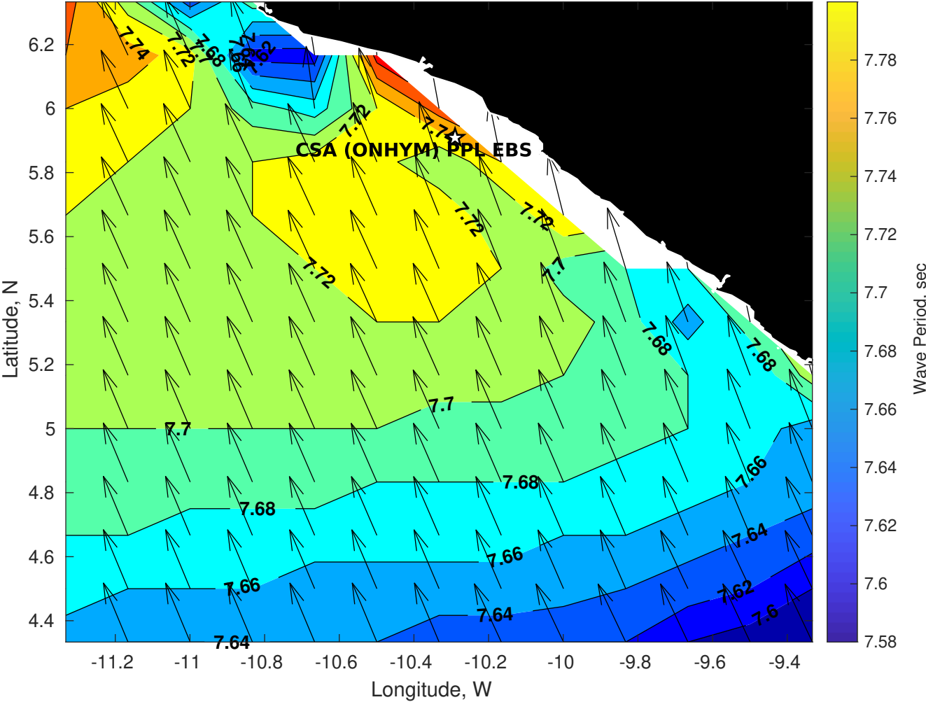
Wave Period (sec) for CSA (ONHYM) PPL EBS - Liberia at 26-Apr-2025 09:00:00
