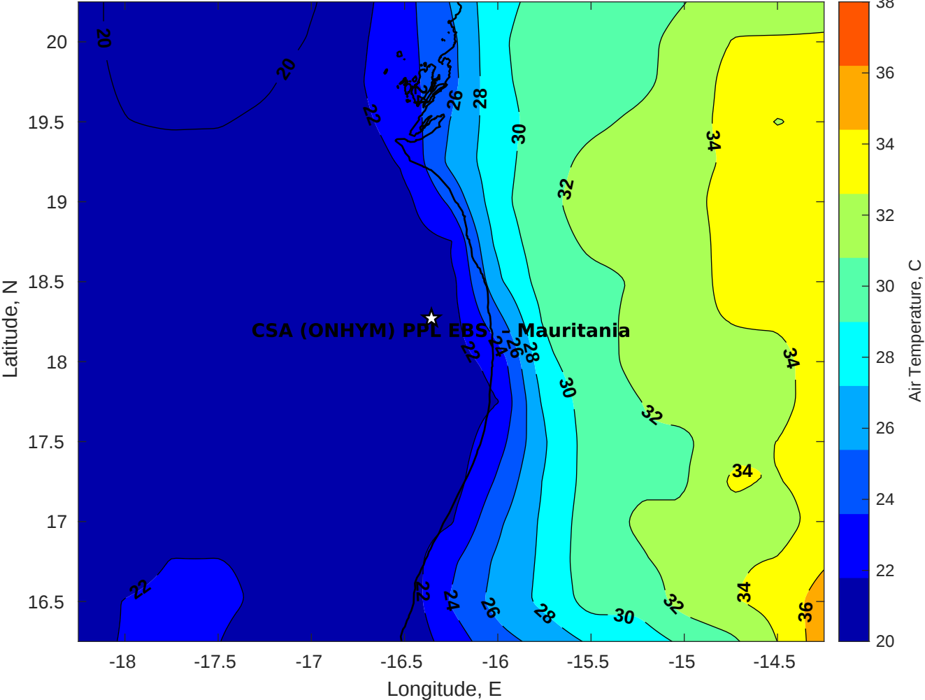
Air Temperature (C) for CSA (ONHYM) PPL EBS - Mauritania at 26-Apr-2025
