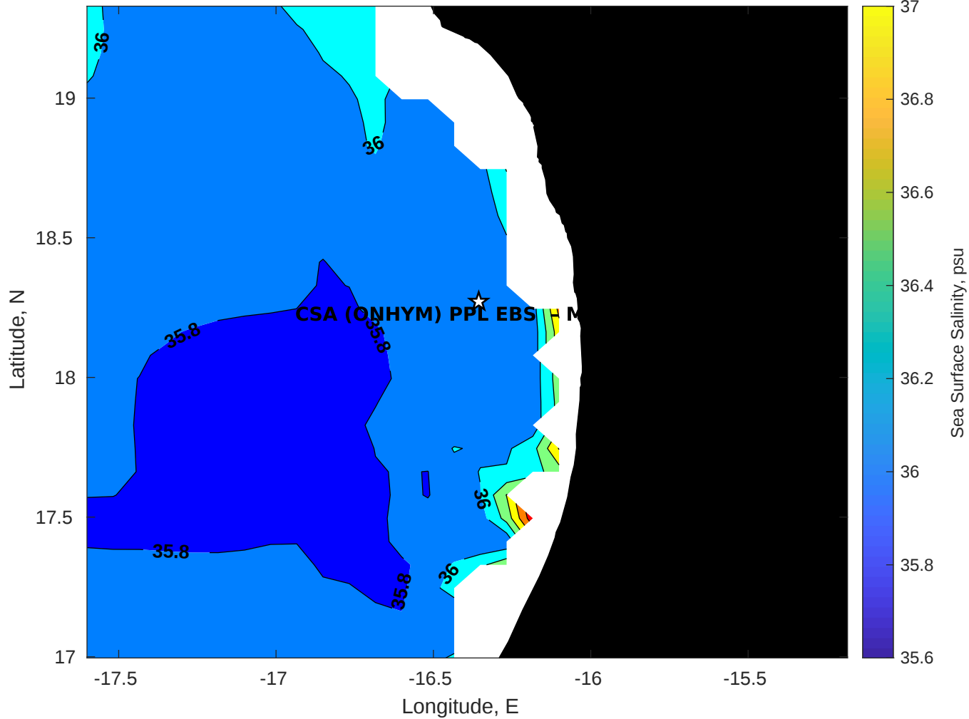
Surface Salinity for CSA (ONHYM) PPL EBS - Mauritania at 25-Apr-2025 00:00:00
