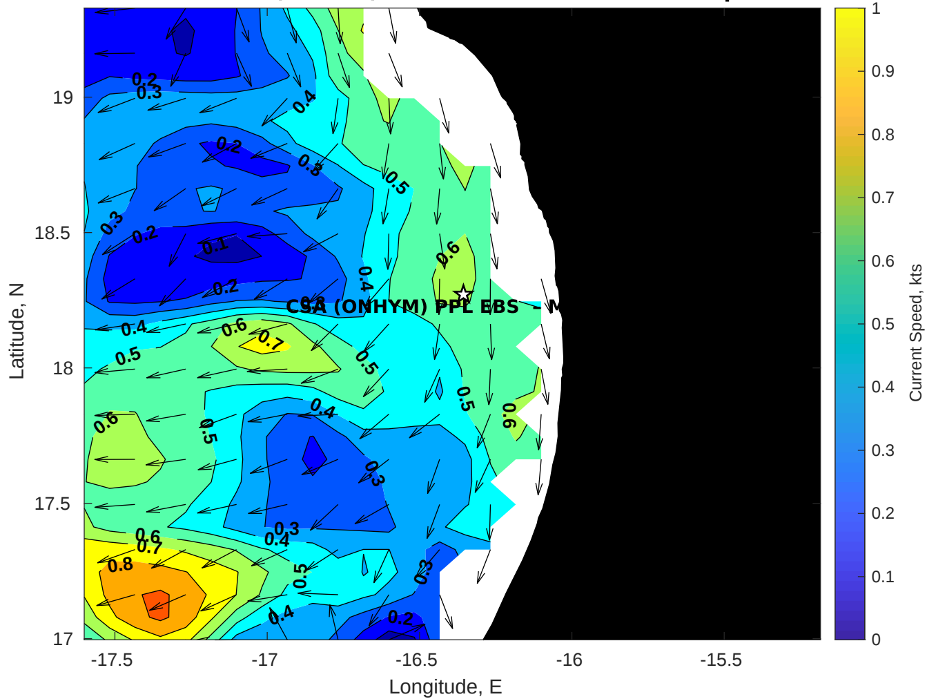
Surface Currents for CSA (ONHYM) PPL EBS - Mauritania at 25-Apr-2025 00:00:00
