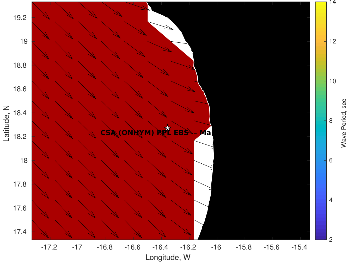
Wave Period (sec) for CSA (ONHYM) PPL EBS - Mauritania at 26-Apr-2025 09:00:00
